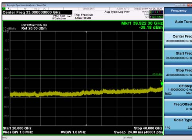
U-NII-1 ,Plot 4,26000MHz~40000MHz-802 .11n(20MHz),5240MHz,Ant1
