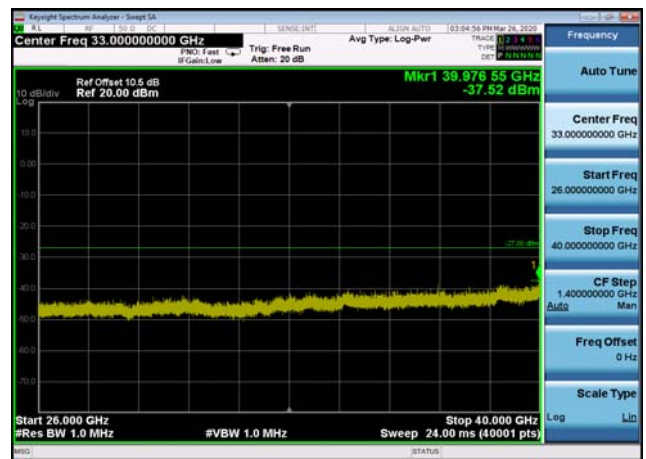
U-NII-1 ,Plot 4,26000MHz~40000MHz-802 .11a(20MHz),5240MHz,Ant1
