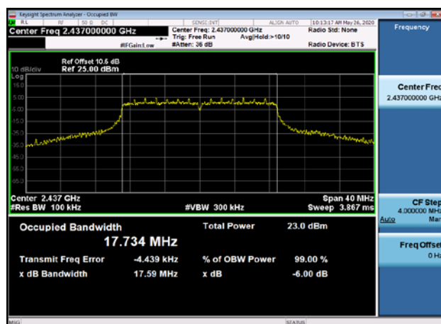
6dB Bandwidth-802.11n(HT20),2437MHz
