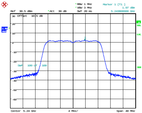
802.11n20_5240MHz
