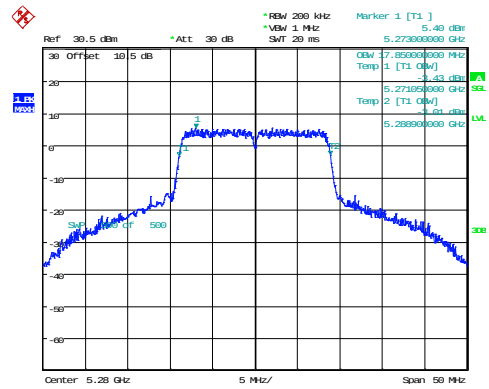
802.11n20_5280MHz
