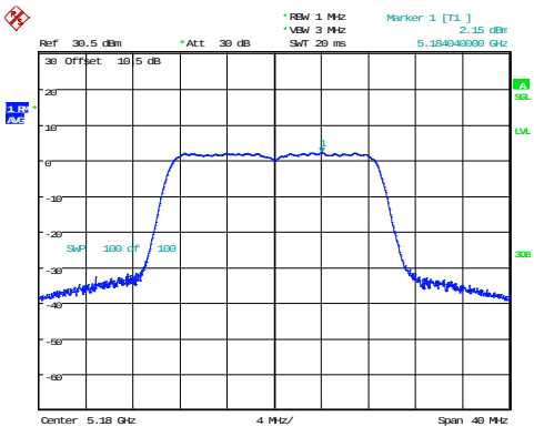
802.11n20_5180MHz
