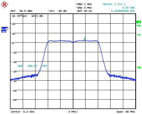
802.11a_5200MHz
