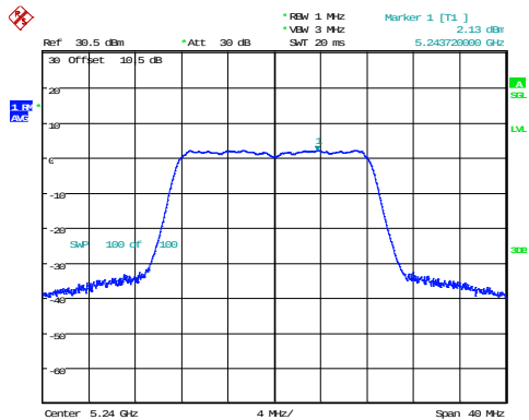
802.11a_5240MHz
