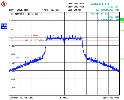
802.11a_5745MHz
