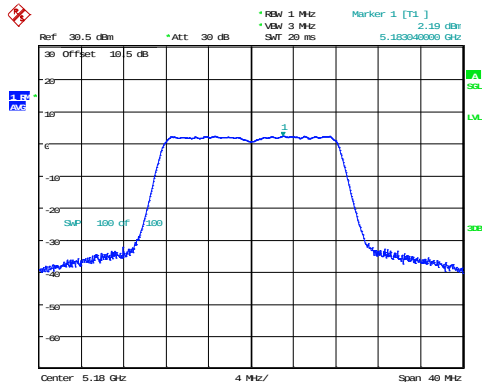
802.11a_5180MHz
