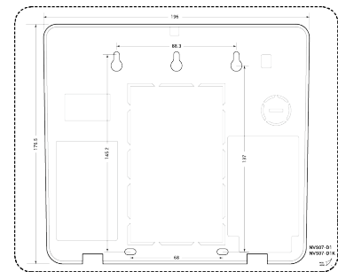
Drilling Template
