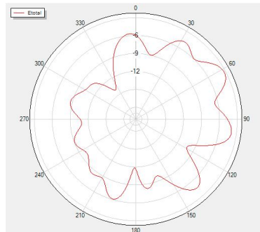
Phi=90 Freq=2450MHz
