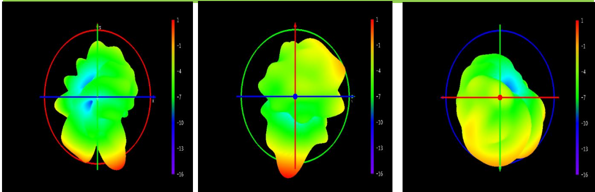
Theta=90 Freq=2450MHz
