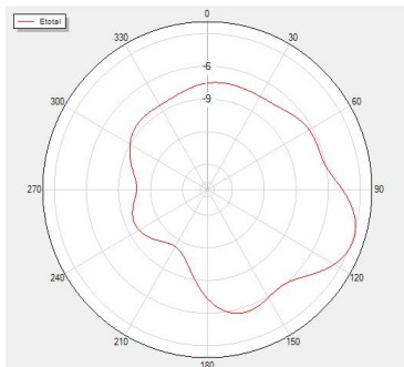
Theta=90 Freq=2450MHz
