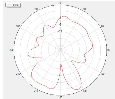
Phi=0 Freq=2450MHz
