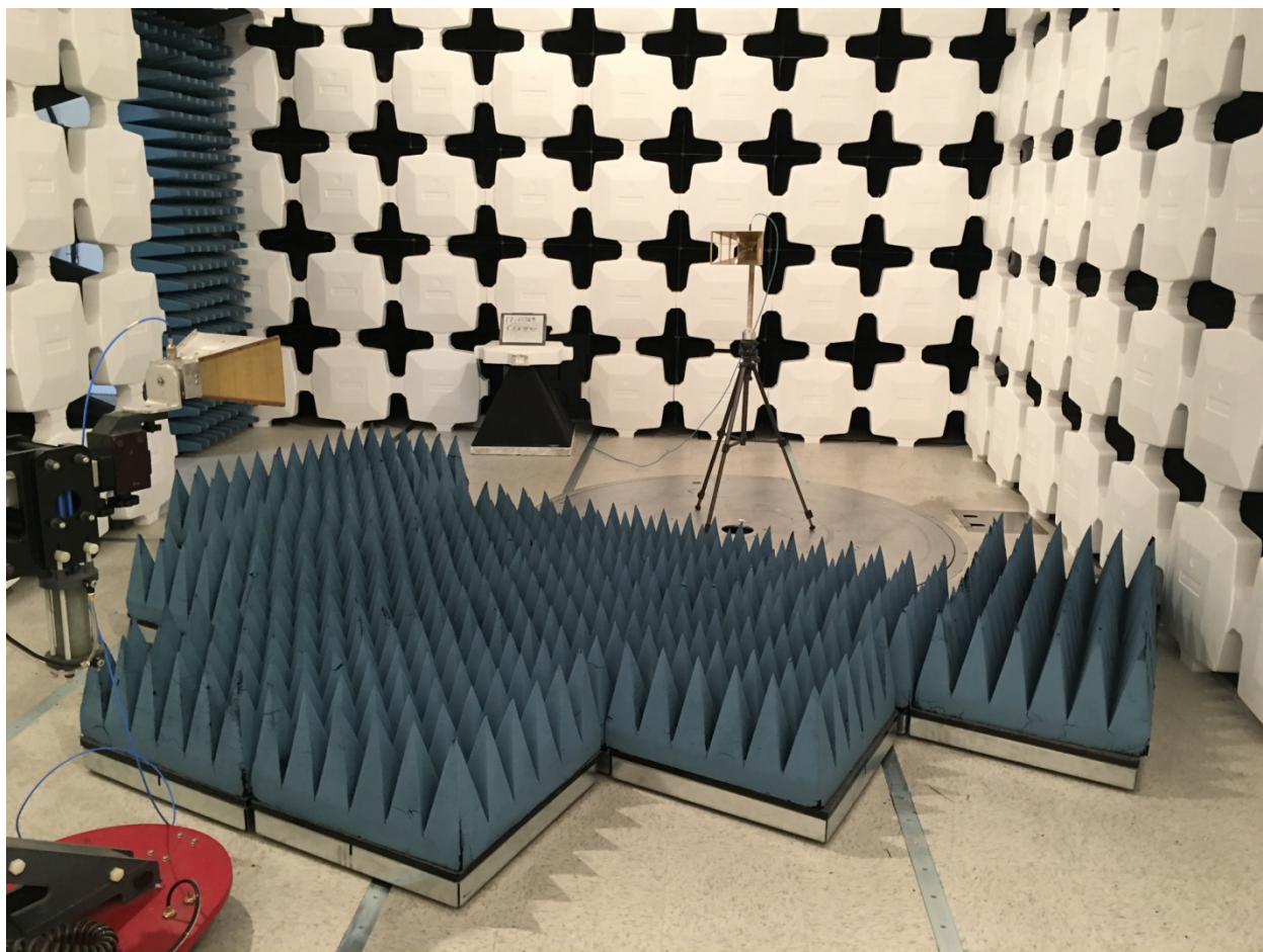
Figure 6. Substitution Setup (above 1 GHz)
