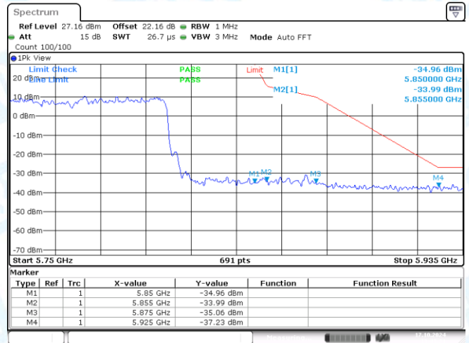
11AX80MIMO-Ant1-5775-PASS
