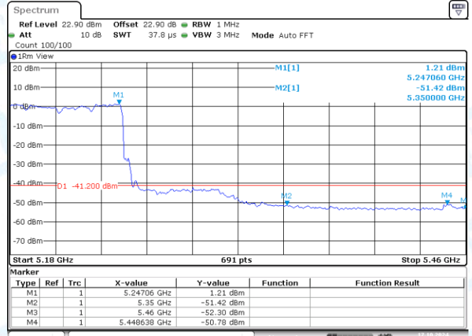
11AX80MIMO-Ant2-5210-PASS
