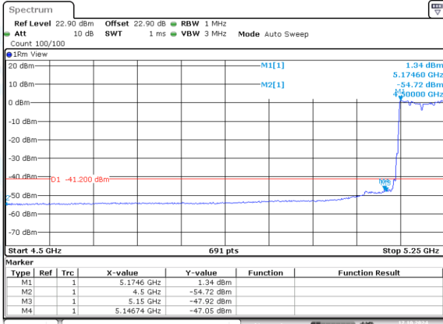
11AX80MIMO-Ant2-5210-PASS
