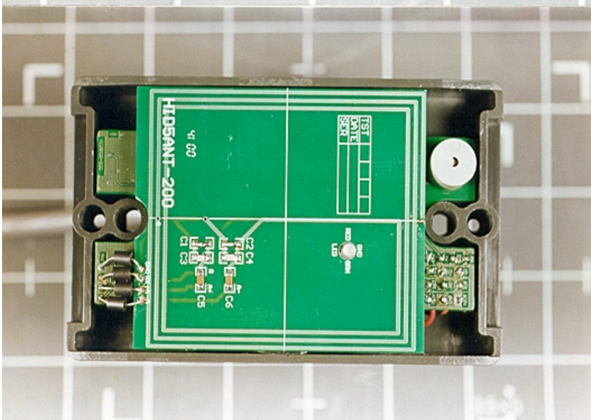
Cover removed
