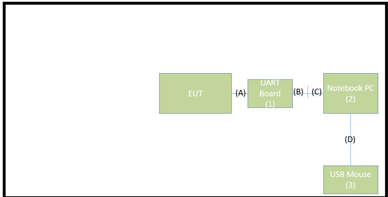
Connection Diagram – Mode1~4
