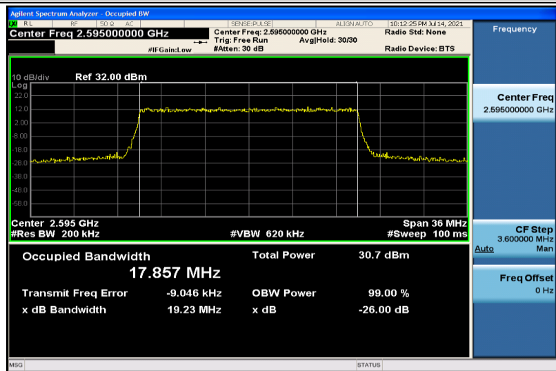
Band38-20MHz-QPSK-38000-100RB#0-17.857
