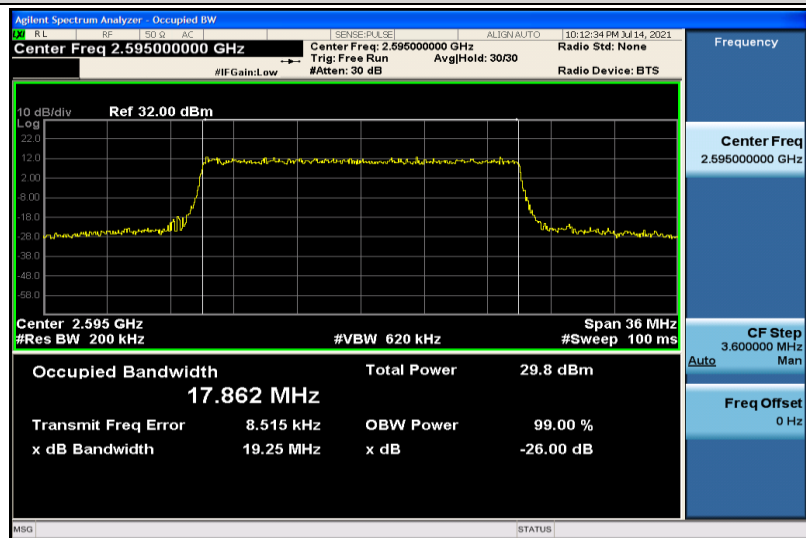
Band38-20MHz-16QAM-38000-100RB#0-17.862
