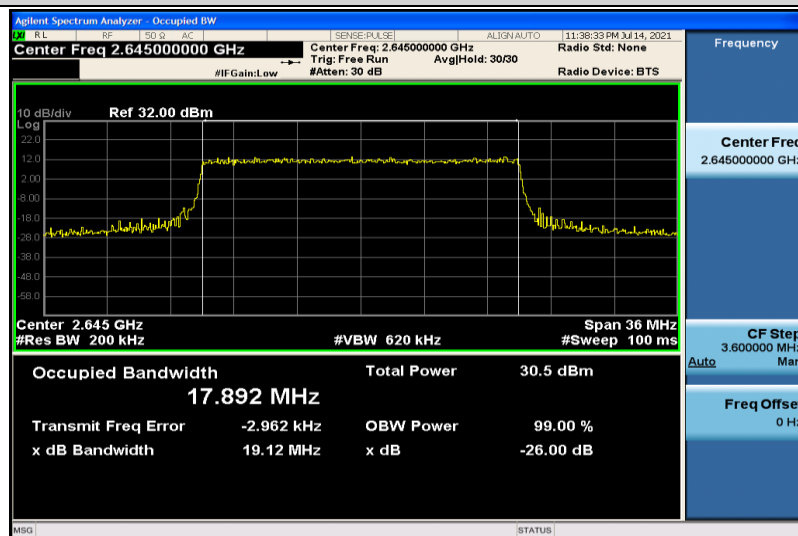
Band41-20MHz-QPSK-41140-100RB#0-17.892
