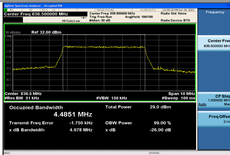
Band5-5MHz-16QAM-20525-25RB#0-4.4851
