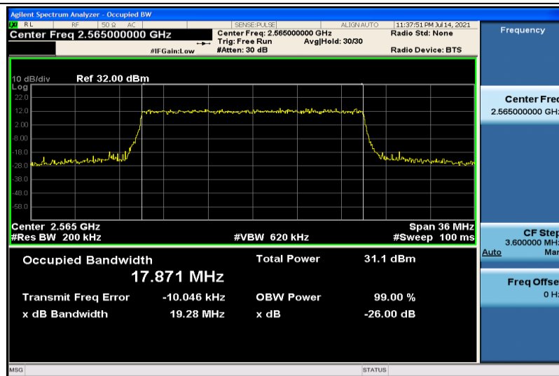
Band41-20MHz-QPSK-40340-100RB#0-17.871
