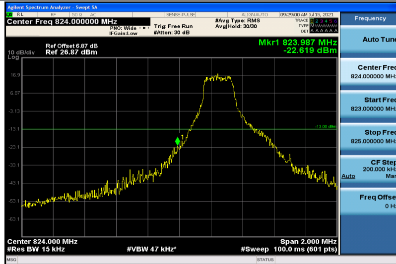
Band5-1.4MHz-QPSK-20407-1RB#0
