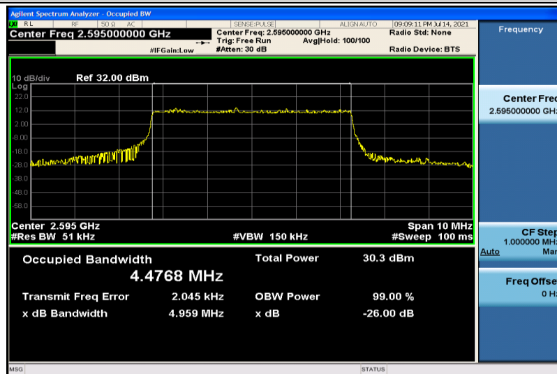
Band38-5MHz-QPSK-38000-25RB#0-4.4768
