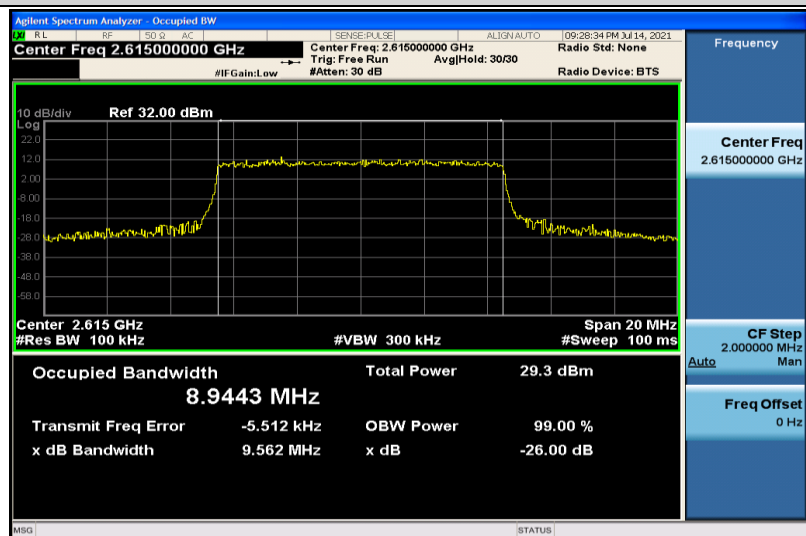
Band38-10MHz-16QAM-38200-50RB#0-8.9443
