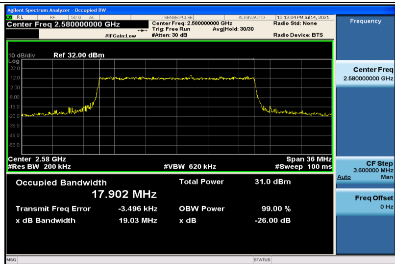
Band38-20MHz-QPSK-37850-100RB#0-17.902
