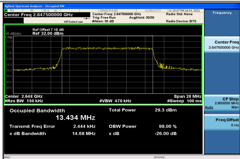
Band41-15MHz-QPSK-41165-75RB#0-13.434
