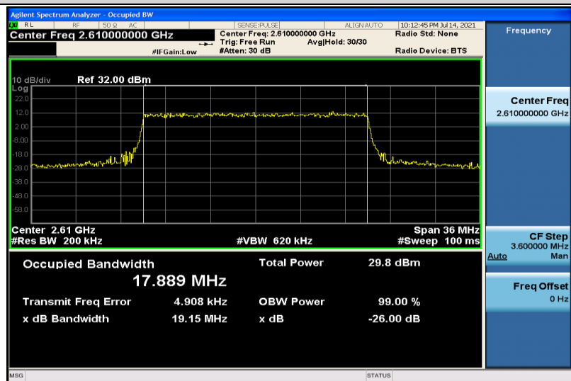
Band38-20MHz-QPSK-38150-100RB#0-17.889
