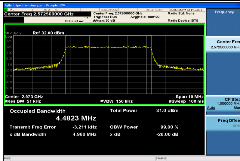
Band38-5MHz-QPSK-37775-25RB#0-4.4823
