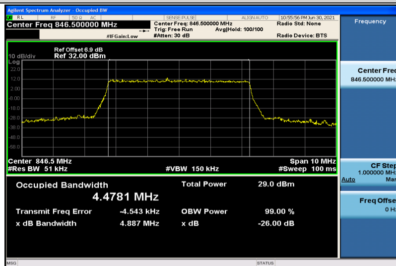
Band5-5MHz-16QAM-20625-25RB#0-4.4781
