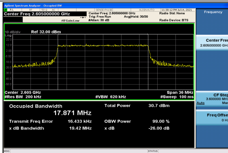
Band41-20MHz-QPSK-40740-100RB#0-17.871
