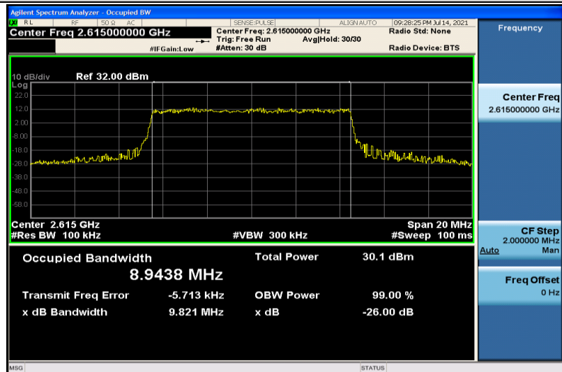
Band38-10MHz-QPSK-38200-50RB#0-8.9438
