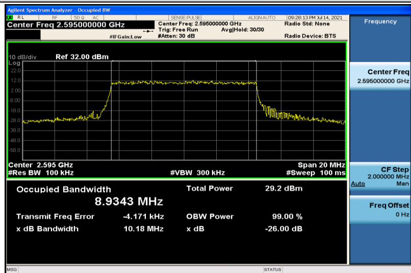
Band38-10MHz-16QAM-38000-50RB#0-8.9343
