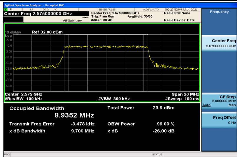
Band38-10MHz-16QAM-37800-50RB#0-8.9352
