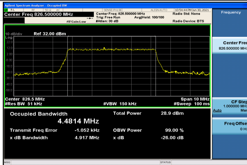
Band5-5MHz-16QAM-20425-25RB#0-4.4814
