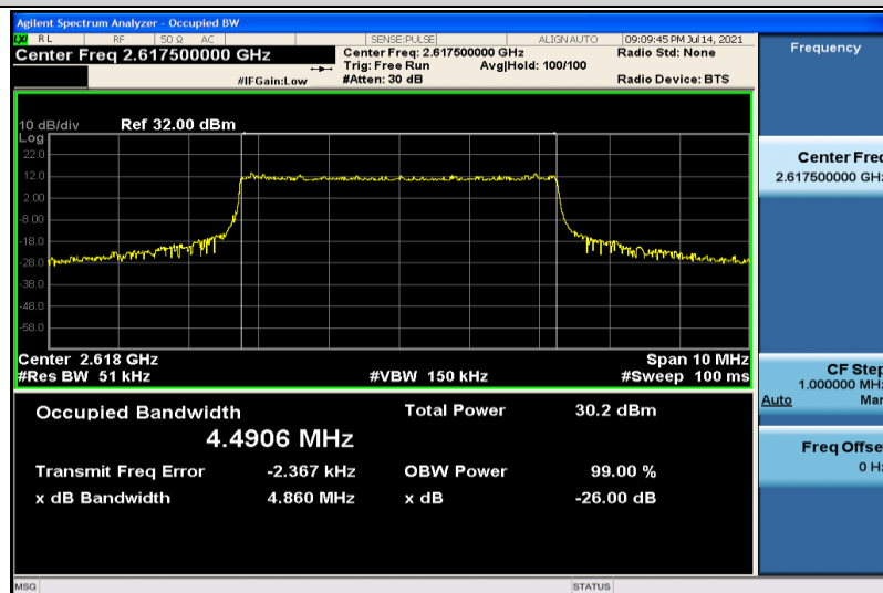
Band38-5MHz-QPSK-38225-25RB#0-4.4906
