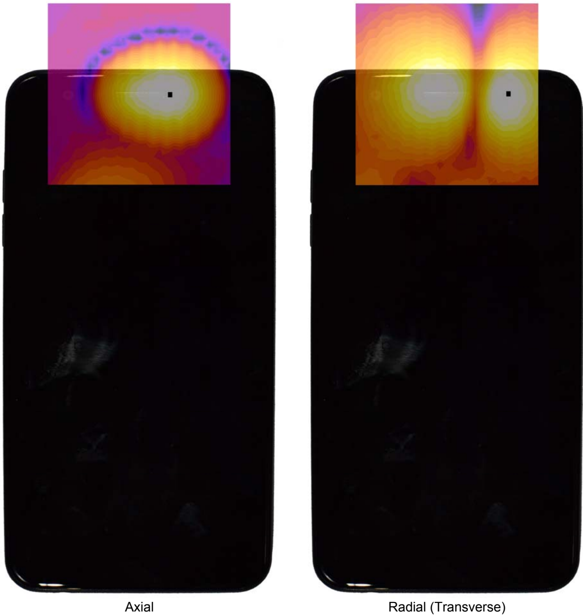
Figure 15-3 T-Coil Scan Overlay Magnetic Field Distributions
