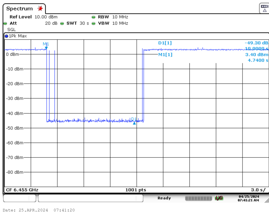
Plot 7-354. Contention Based Protocol Timing Plot (20MHz (UNII Band 6) – Ch. 101)
