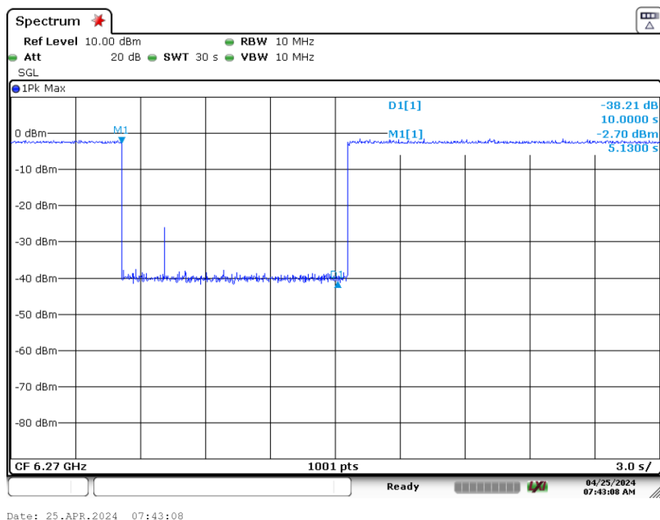
Plot 7-355. Contention Based Protocol Timing Plot (320MHz (UNII Band 6) – Ch. 95 Low)
