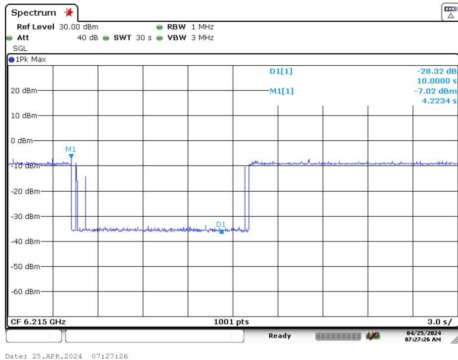
Plot 7-350. Contention Based Protocol Timing Plot (20MHz (UNII Band 5) – Ch. 53)
