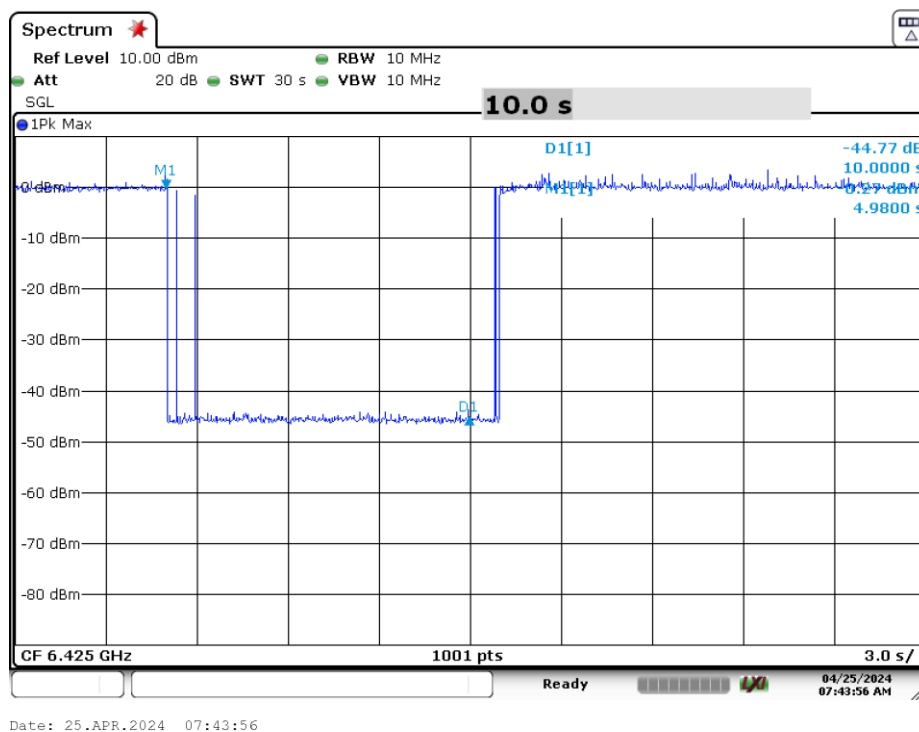
Plot 7-356. Contention Based Protocol Timing Plot (320MHz (UNII Band 6) – Ch. 95 Mid)
