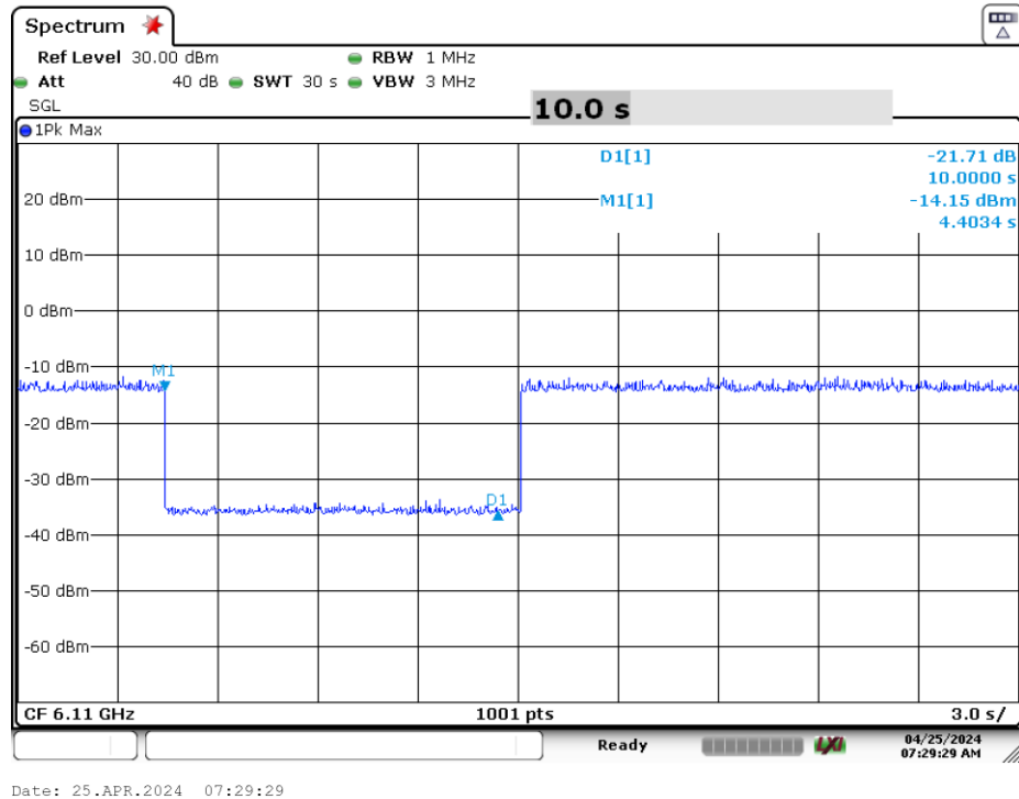
Plot 7-351. Contention Based Protocol Timing Plot (320MHz (UNII Band 5) – Ch. 31 Low)
