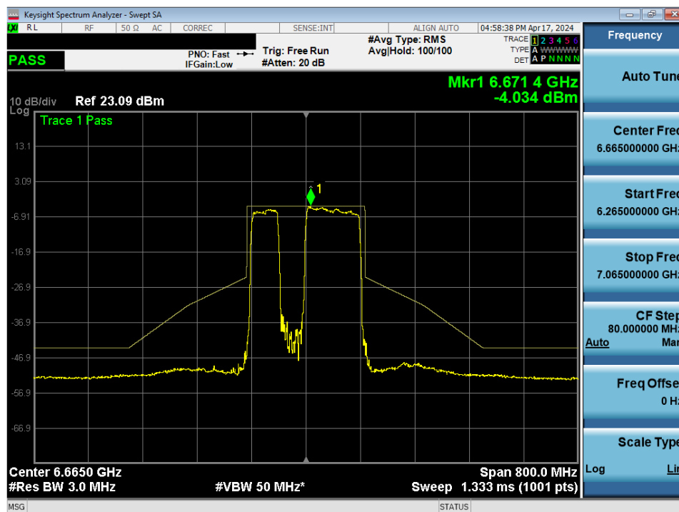
Plot 7-329. In-Band Emission Plot MIMO ANT2 (160MHz BW 802.11be (996+484 Tone) (UNII Band 7) – Ch. 143) – LPI&SP
