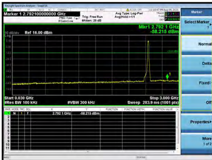
802.11g CHANNEL 10, SPURIOUS 30 MHz ~ 3 GHz
