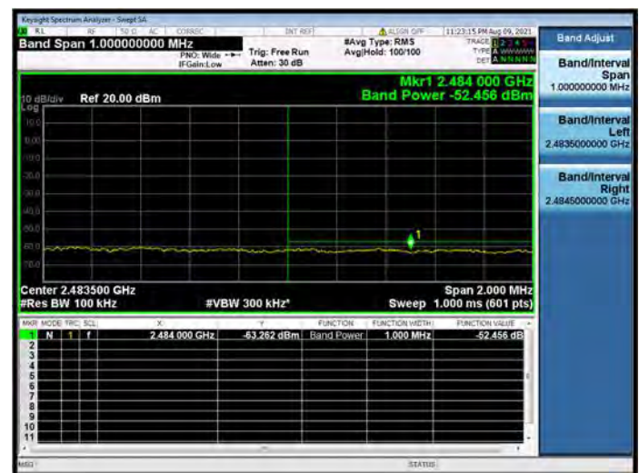
802.11n-20 MHz CHANNEL 10, Reference level
