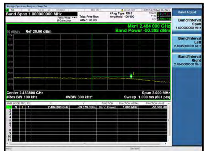
802.11b CHANNEL 10, Reference level
