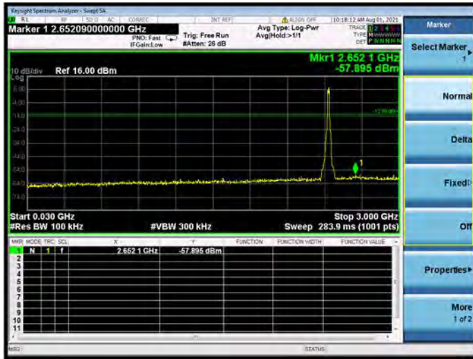
802.11g CHANNEL 6, SPURIOUS 30 MHz ~ 3 GHz
