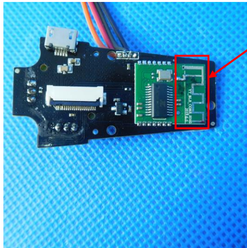
RF Antenna
