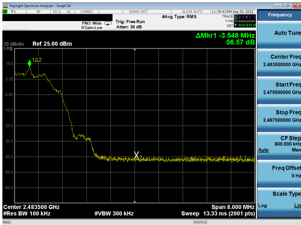
Plot 7-62. Band Edge Plot (Bluetooth (LE), 2Mbps – Ch. 39)
