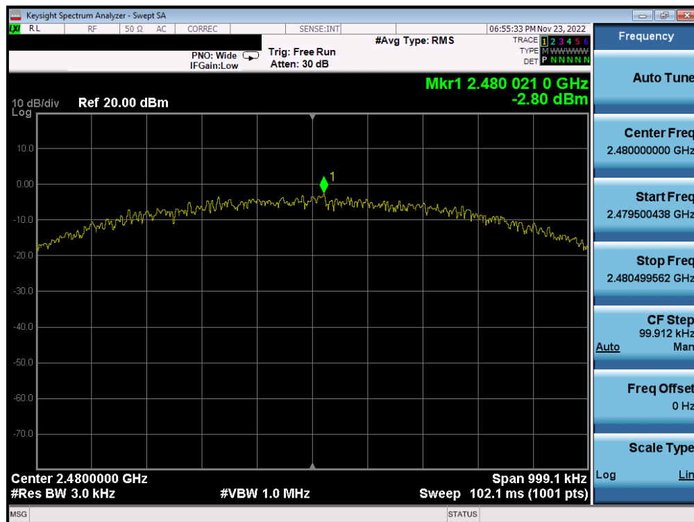
Plot 7-51. Power Spectral Density Plot (Bluetooth (LE), 1Mbps – Ch. 039Ant2)
