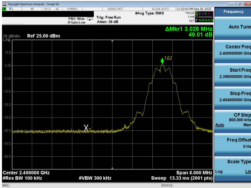
Plot 7-55. Band Edge Plot (Bluetooth (LE), 125kbps – Ch. 0)
