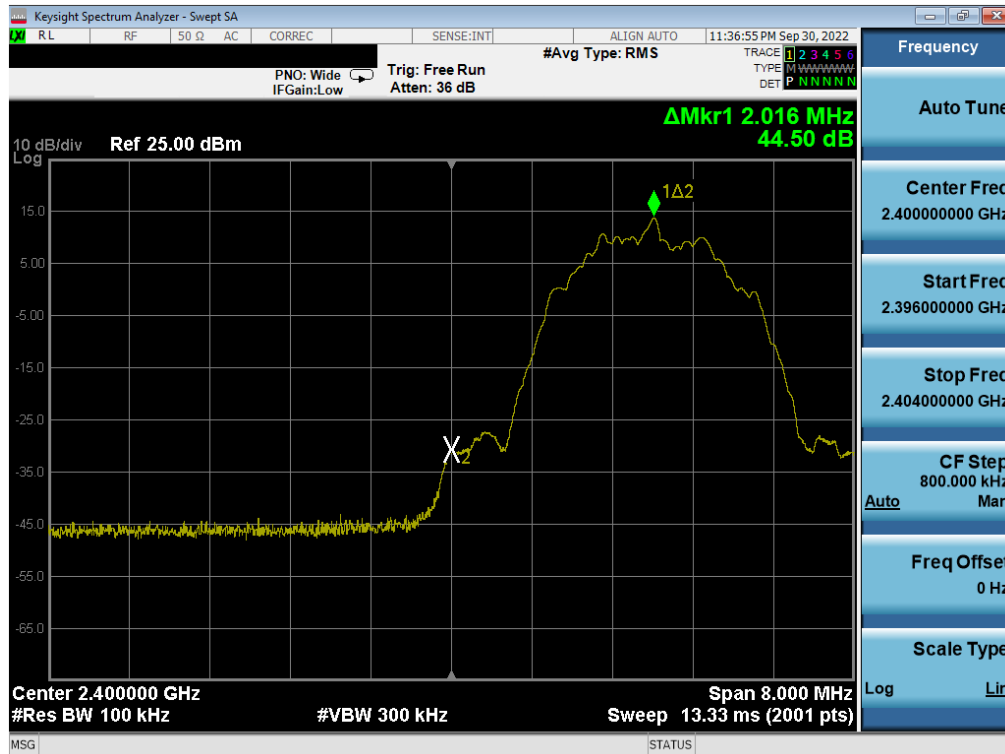
Plot 7-65. Band Edge Plot (Bluetooth (LE), 2Mbps – Ch. 0)
