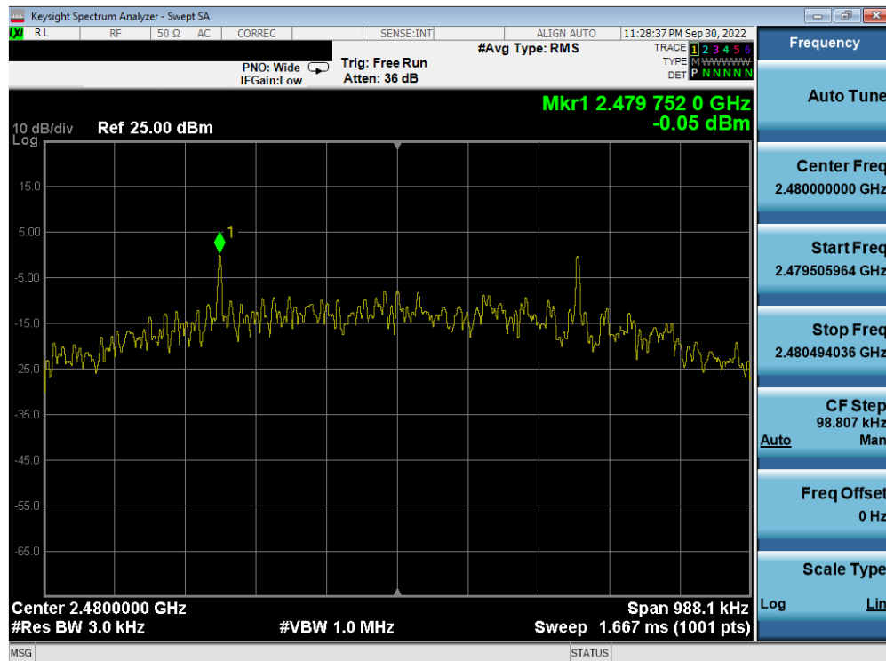
Plot 7-42. Power Spectral Density Plot (Bluetooth (LE), 500kbps – Ch. 39) Ant1
