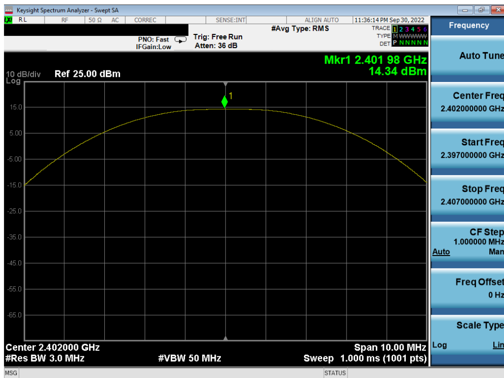
Plot 7-28. Peak Power Plot (Bluetooth (LE), 2Mbps – Ch. 0) Ant1
