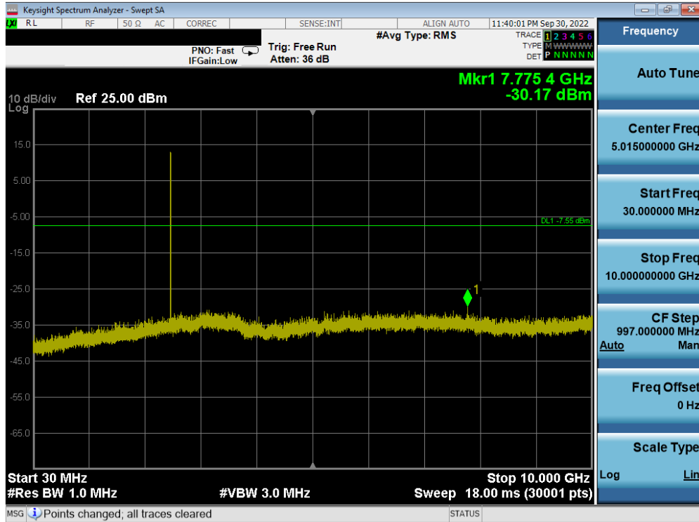
Plot 7-71. Conducted Spurious Plot (Bluetooth (LE), 2Mbps – Ch. 39) Ant1
