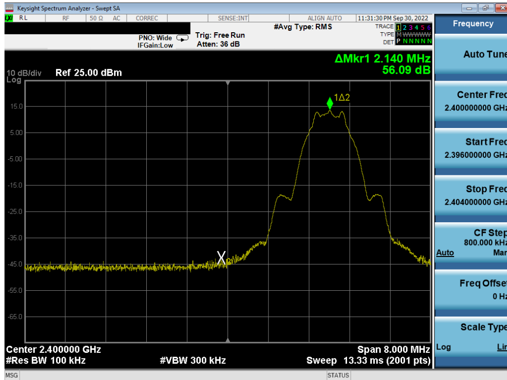
Plot 7-63. Band Edge Plot (Bluetooth (LE), 1Mbps – Ch. 0)
