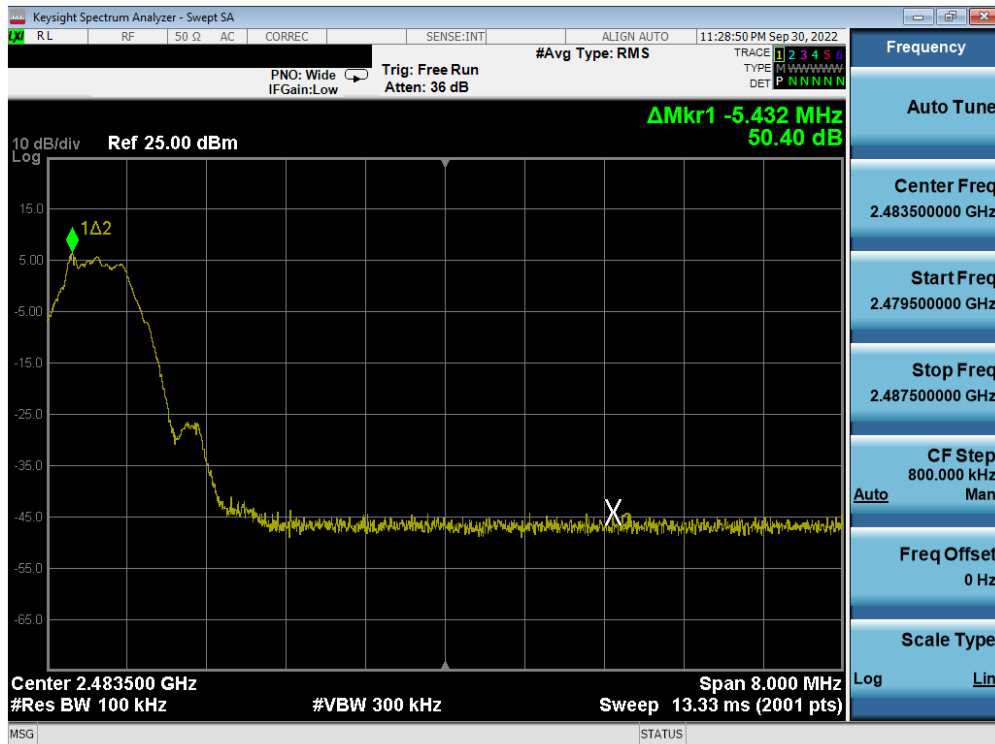
Plot 7-58. Band Edge Plot (Bluetooth (LE), 500kbps – Ch. 39)
