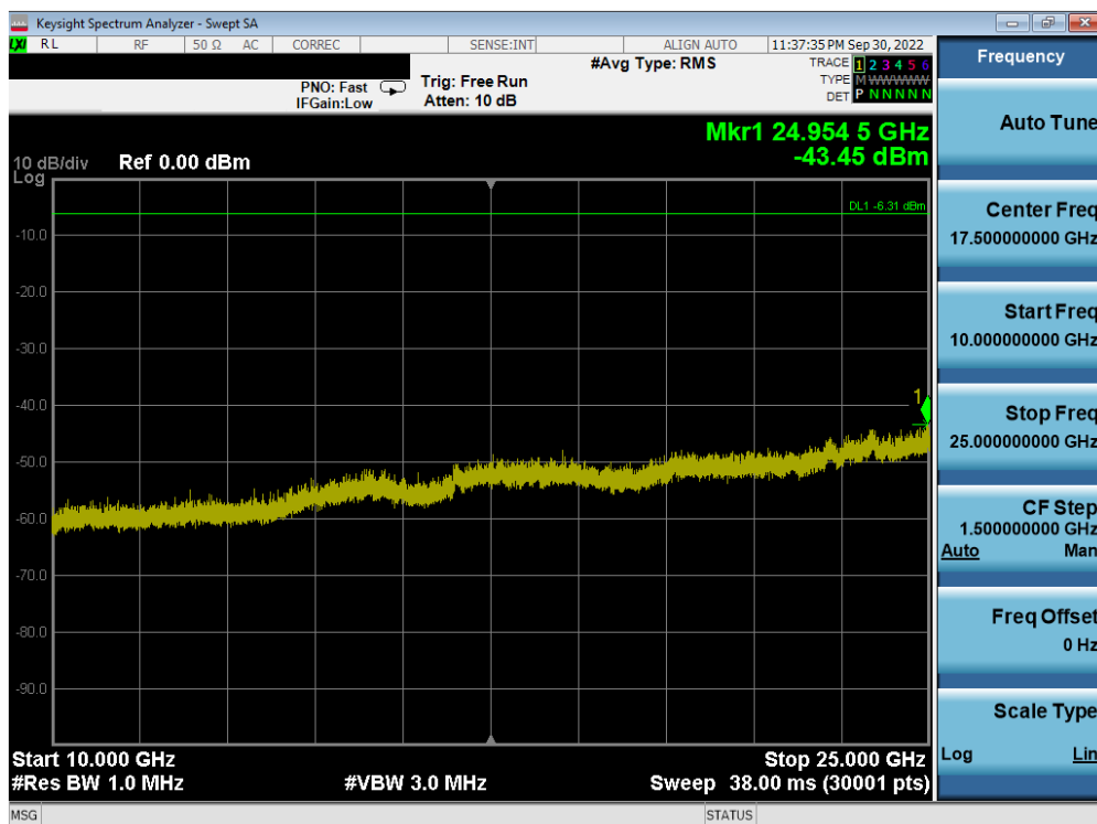
Plot 7-68. Conducted Spurious Plot (Bluetooth (LE), 2Mbps – Ch. 0) Ant1
