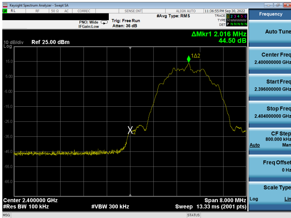
Plot 7-61. Band Edge Plot (Bluetooth (LE), 2Mbps – Ch. 0)
