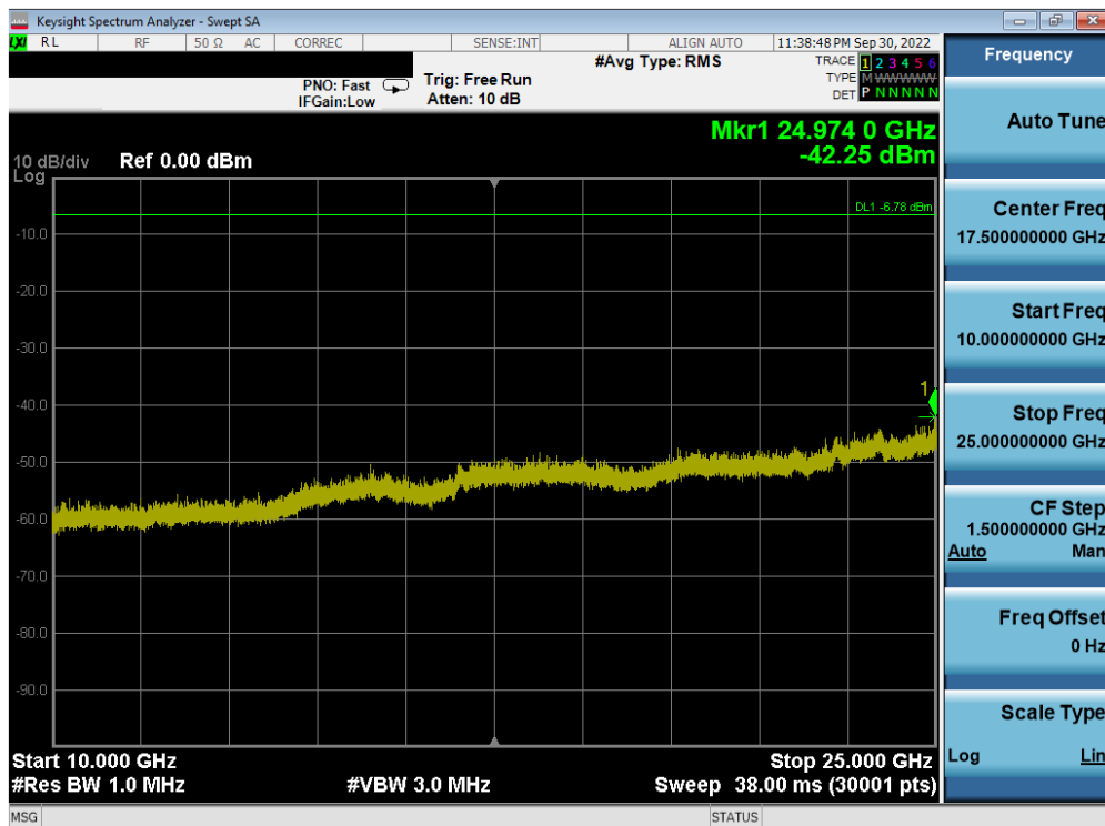
Plot 7-70. Conducted Spurious Plot (Bluetooth (LE), 2Mbps – Ch. 19) Ant1
