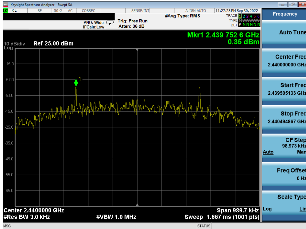
Plot 7-41. Power Spectral Density Plot (Bluetooth (LE), 500kbps – Ch. 19) Ant1
