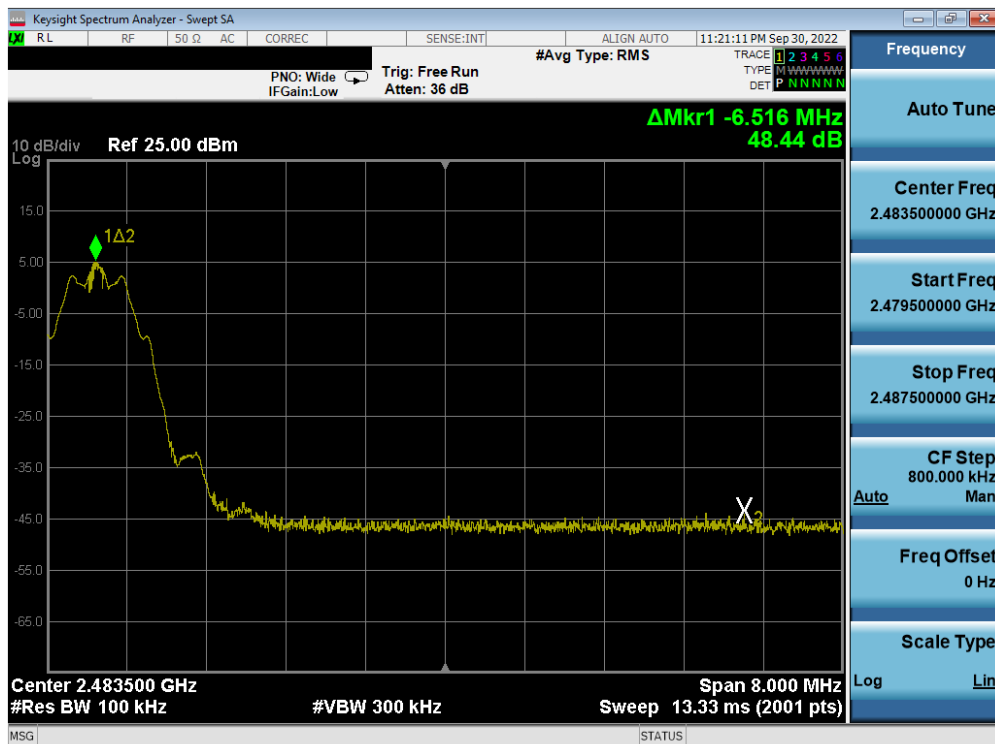
Plot 7-56. Band Edge Plot (Bluetooth (LE), 125kbps – Ch. 39)
