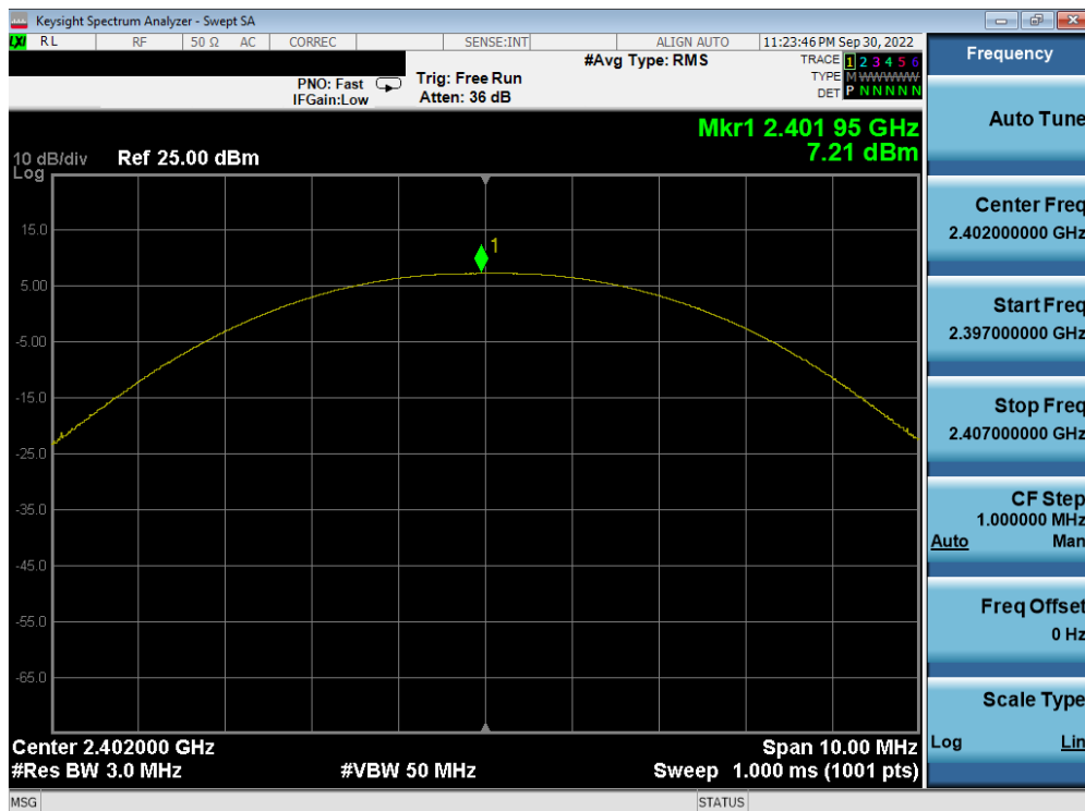
Plot 7-22. Peak Power Plot (Bluetooth (LE), 500kbps – Ch. 0) Ant1
