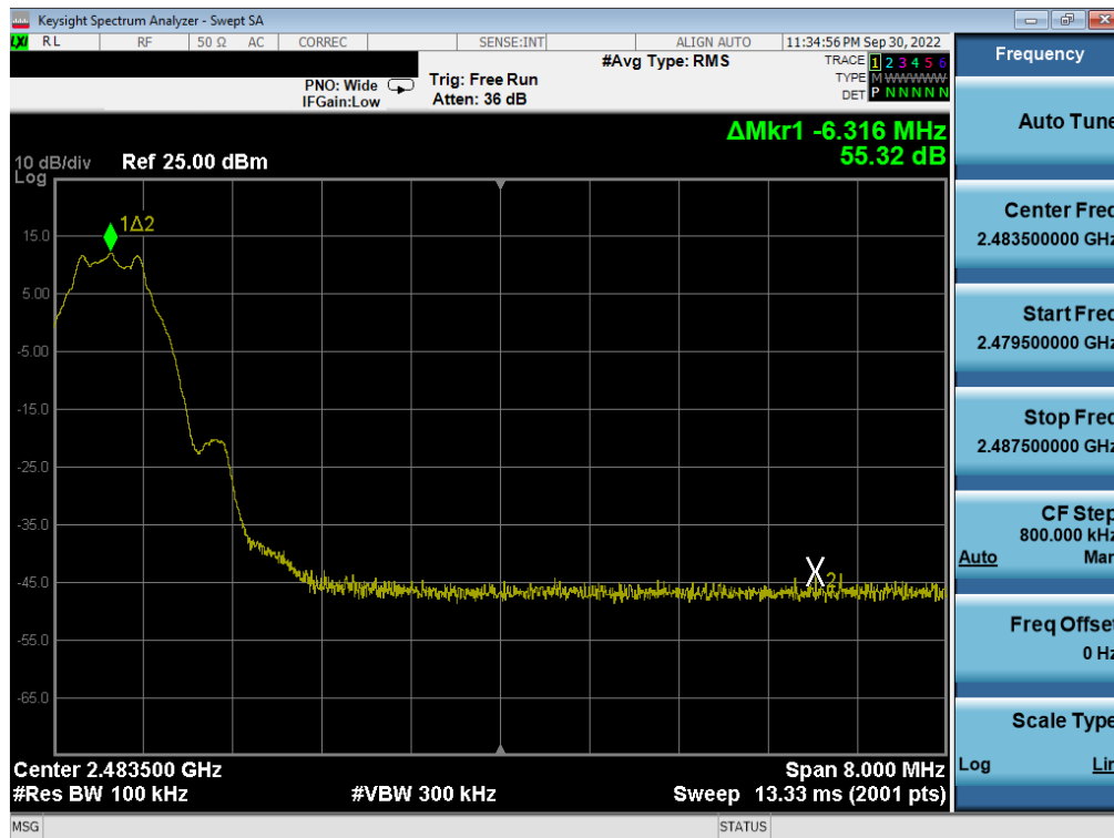
Plot 7-60. Band Edge Plot (Bluetooth (LE), 1Mbps – Ch. 39)
