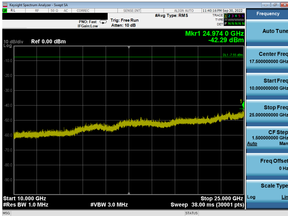
Plot 7-72. Conducted Spurious Plot (Bluetooth (LE), 2Mbps – Ch. 39) Ant1
