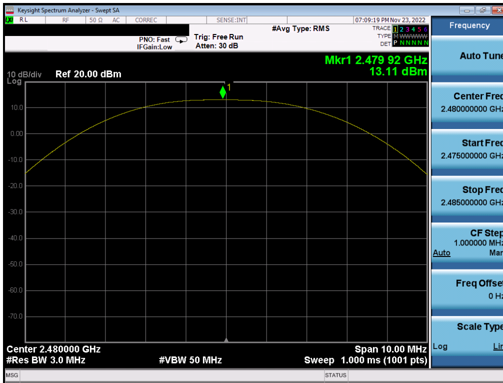
Plot 7-36. Peak Power Plot (Bluetooth (LE), 2Mbps – Ch. 39) Ant2
