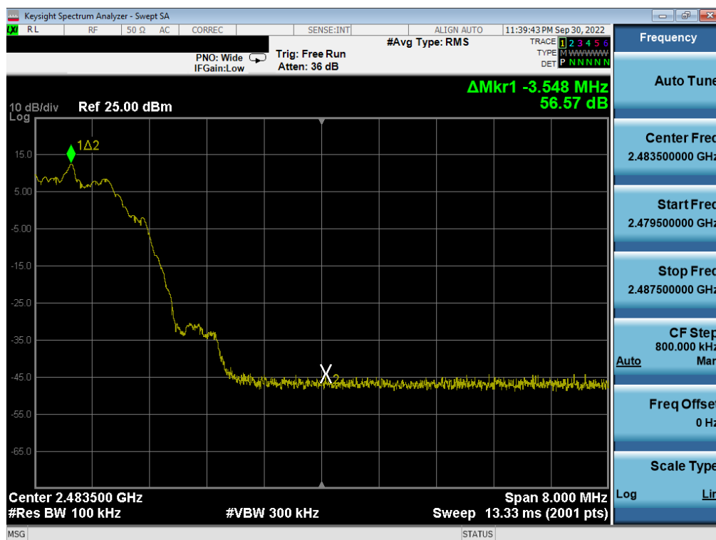
Plot 7-66. Band Edge Plot (Bluetooth (LE), 2Mbps – Ch. 39)
