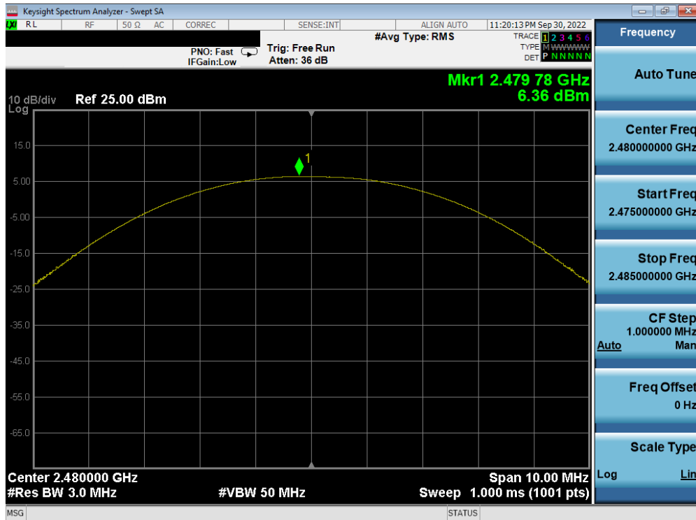
Plot 7-21. Peak Power Plot (Bluetooth (LE), 125kbps – Ch. 39) Ant1
