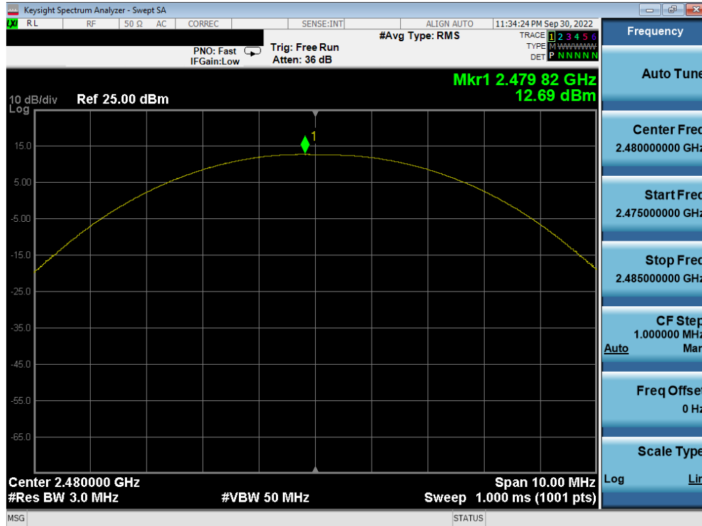
Plot 7-27. Peak Power Plot (Bluetooth (LE), 1Mbps – Ch. 39) Ant1
