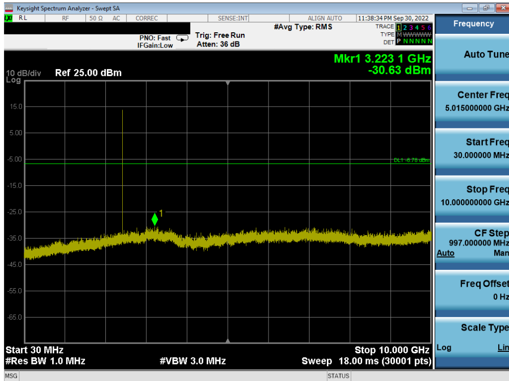
Plot 7-69. Conducted Spurious Plot (Bluetooth (LE), 2Mbps – Ch. 19) Ant1
