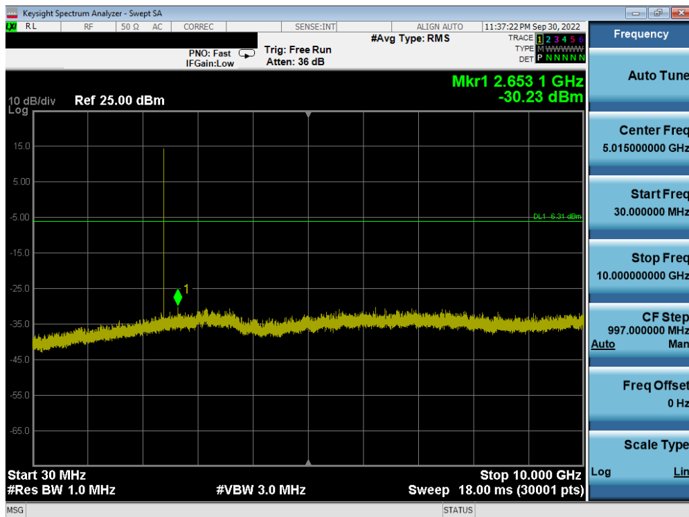
Plot 7-67. Conducted Spurious Plot (Bluetooth (LE), 2Mbps – Ch. 0) Ant1
