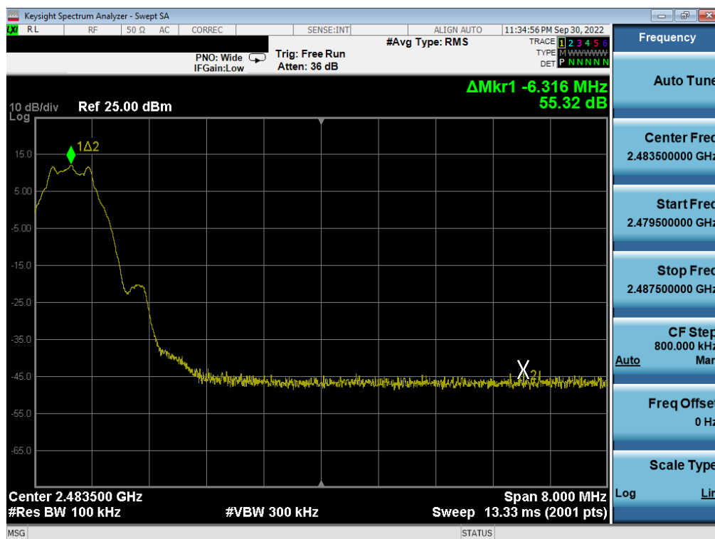
Plot 7-64. Band Edge Plot (Bluetooth (LE), 1Mbps – Ch. 39)
