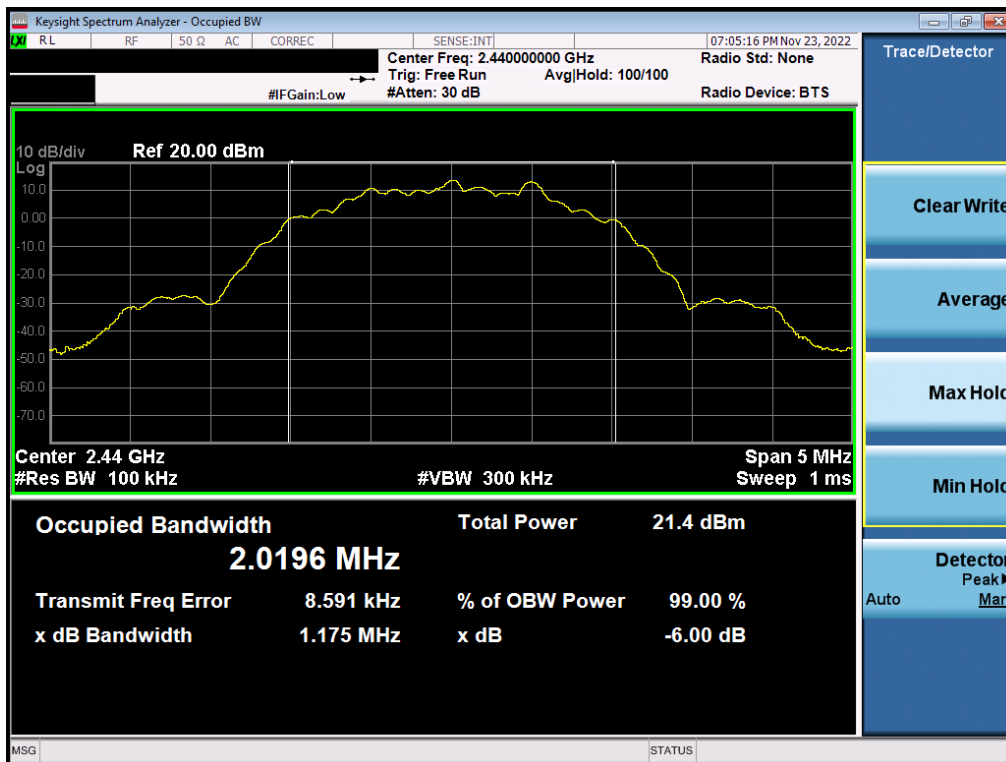
Plot 7-17. 6dB Bandwidth Plot (Bluetooth (LE), 2Mbps – Ch. 19) ANT2
