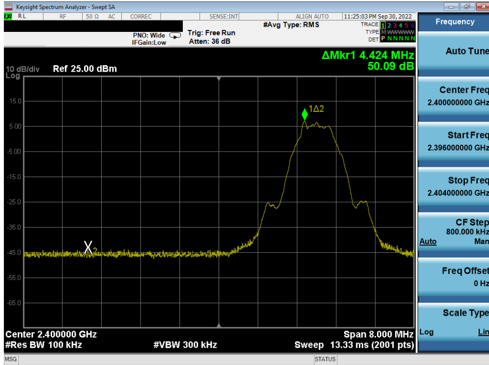
Plot 7-57. Band Edge Plot (Bluetooth (LE), 500kbps – Ch. 0)
