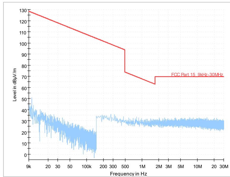
Fig. 109 Radiated Spurious Emission (All Channel, 9 kHz ~30 MHz)
