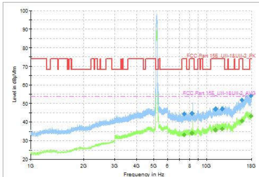
Fig. 101 Transmitter Spurious Emission (802.11ac-VHT80, CH42 5210MHz, 1GHz-18GHz)
