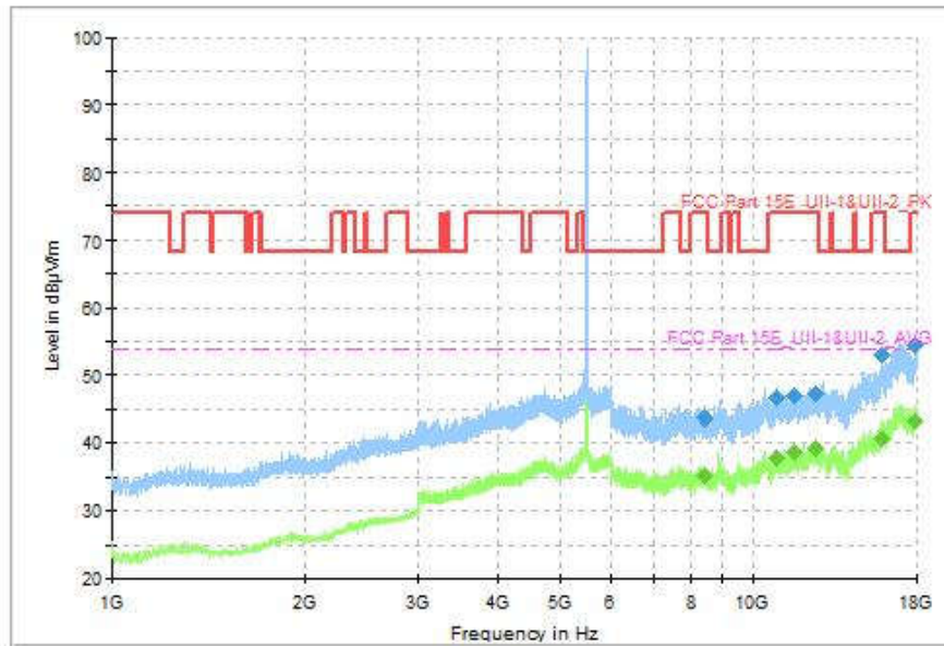
Fig. 96 Transmitter Spurious Emission (802.11ac-VHT40, CH102 5510MHz, 1GHz-18GHz)
