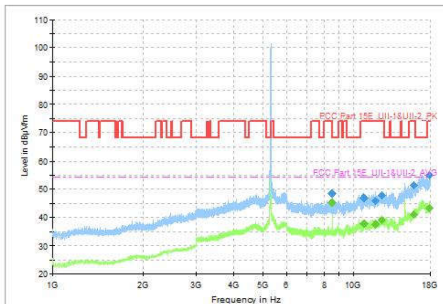
Fig. 95 Transmitter Spurious Emission (802.11ac-VHT40, CH62 5310MHz, 1GHz-18GHz)
