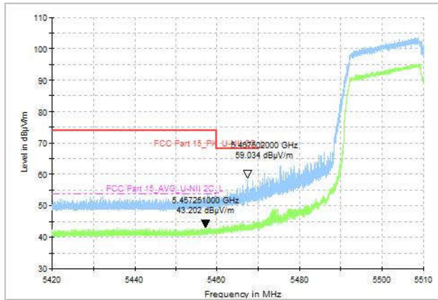
Fig. 71 Band Edges (802.11ac-VHT40, CH102 5510MHz)
