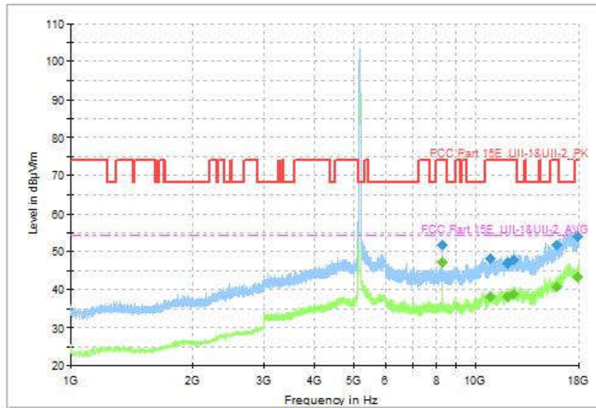
Fig. 92 Transmitter Spurious Emission (802.11ac-VHT40, CH38 5190MHz, 1GHz-18GHz)
