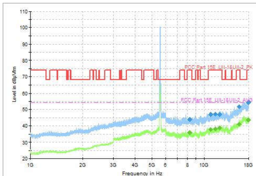
Fig. 97 Transmitter Spurious Emission (802.11ac-VHT40, CH118 5580MHz, 1GHz-18GHz)
