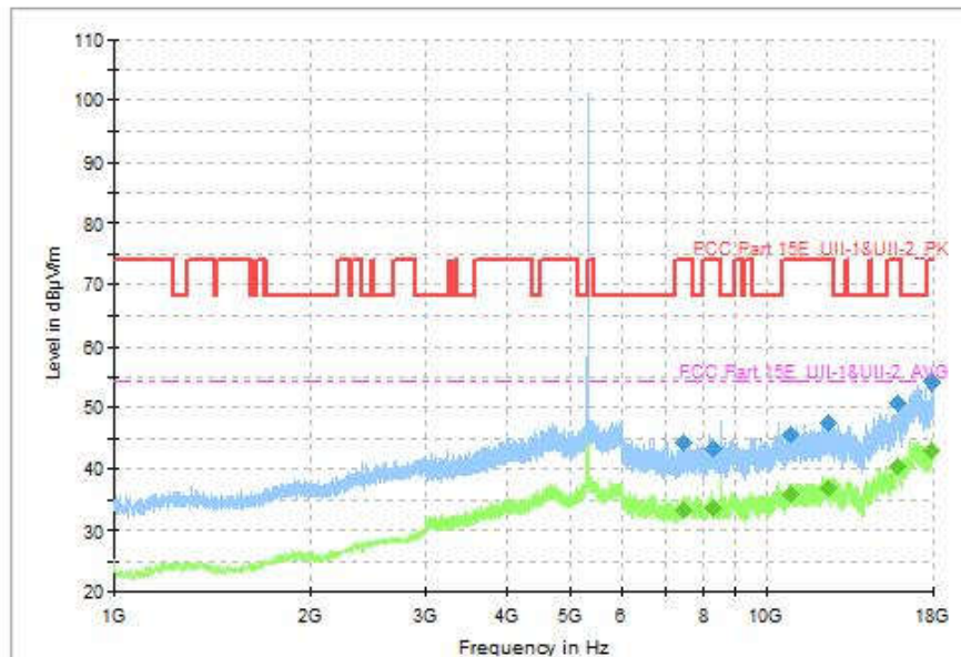
Fig. 85 Transmitter Spurious Emission (802.11a, CH64 5320MHz, 1GHz-18GHz)
