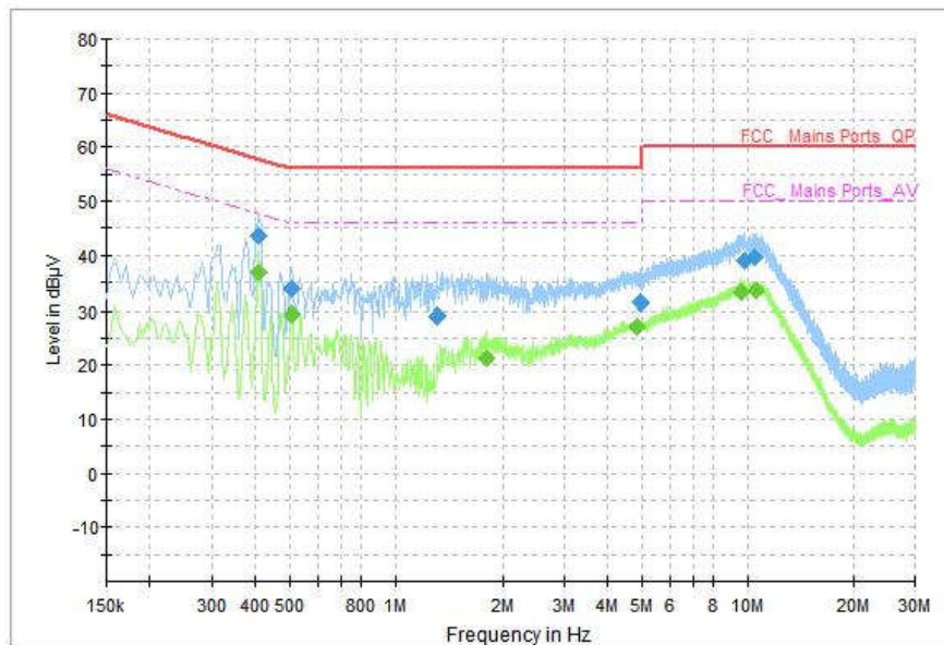
Fig. 111 AC Power line Conducted Emission (Idle)
