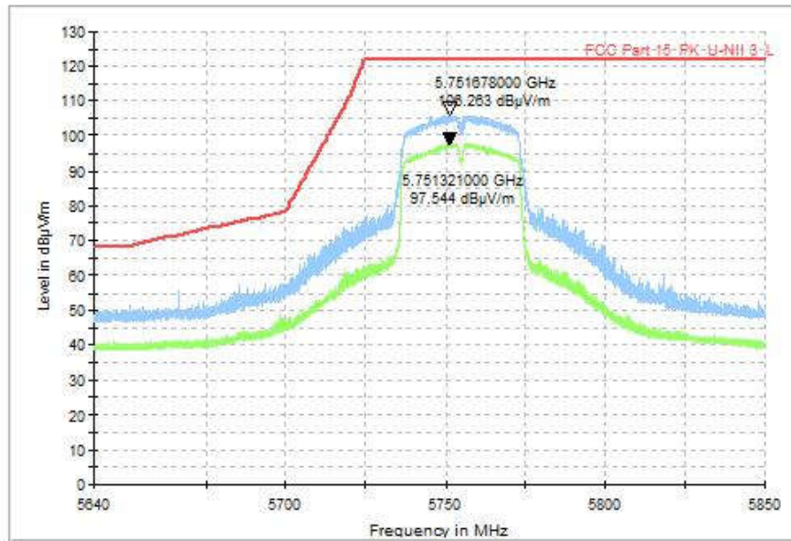
Fig. 73 Band Edges (802.11ac-VHT40, CH151 5755MHz)
