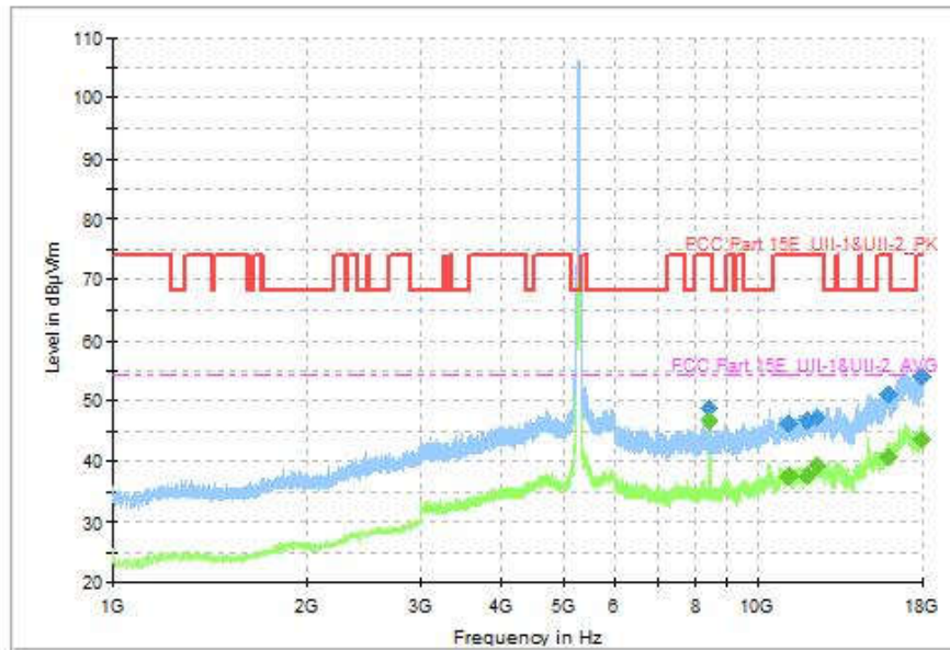
Fig. 94 Transmitter Spurious Emission (802.11ac-VHT40, CH54 5270MHz, 1GHz-18GHz)
