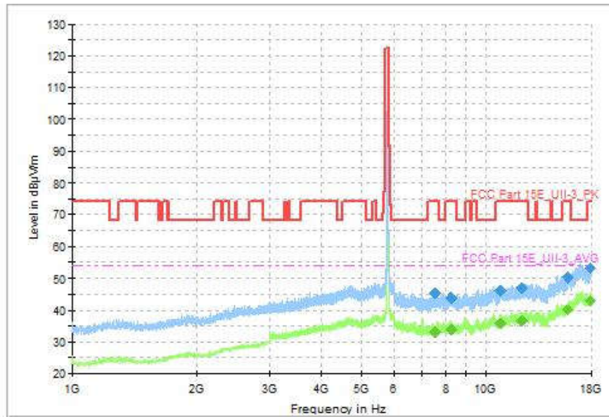
Fig. 100 Transmitter Spurious Emission (802.11ac-VHT40, CH159 5795MHz, 1GHz-18GHz)
