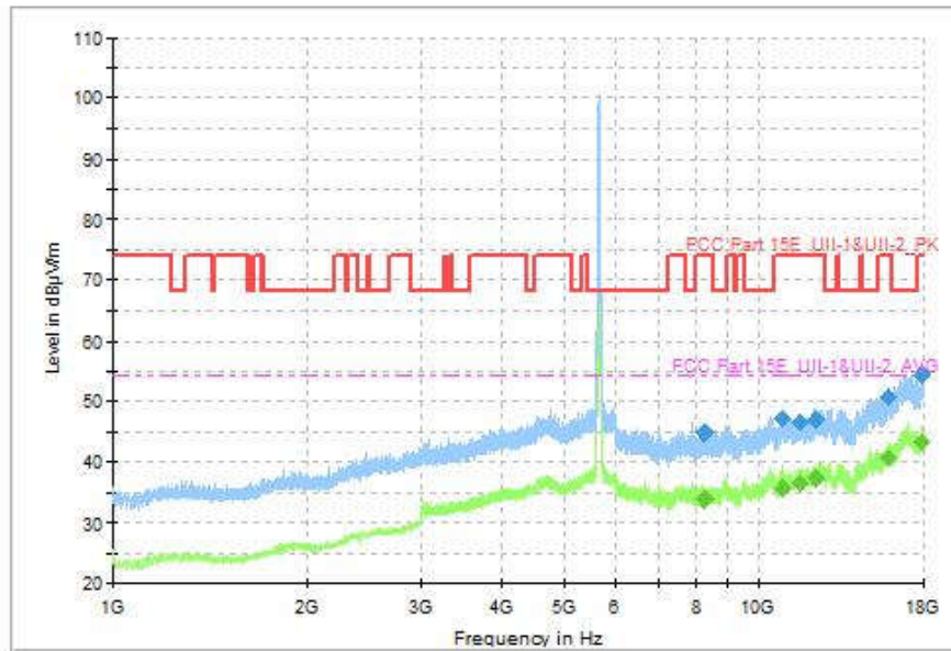
Fig. 98 Transmitter Spurious Emission (802.11ac-VHT40, CH134 5670MHz, 1GHz-18GHz)
