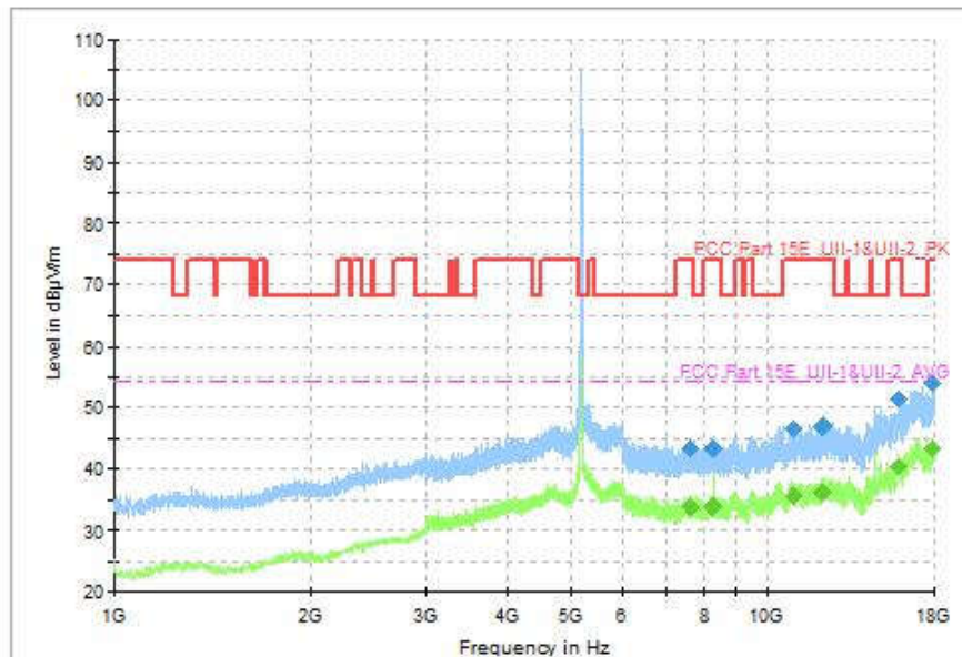
Fig. 81 Transmitter Spurious Emission (802.11a, CH40 5200MHz, 1GHz-18GHz)
