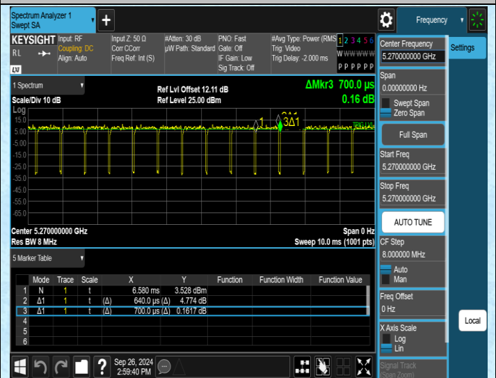
NTNV-11N40MIMO-Ant2-5270
