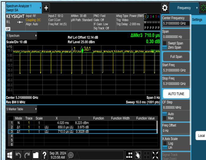
NTNV-11AC40SISO-Ant1-5310
