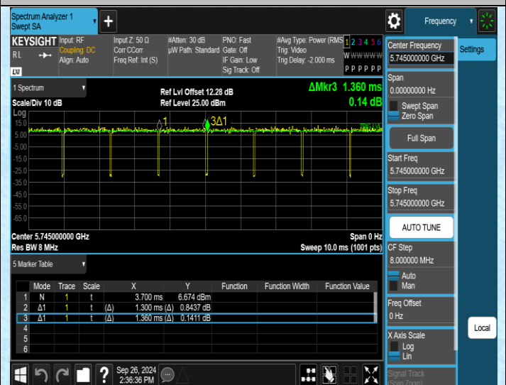
NTNV-11N20MIMO-Ant2-5745
