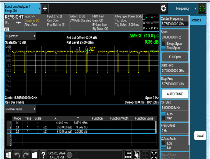
NTNV-11AC40SISO-Ant2-5755
