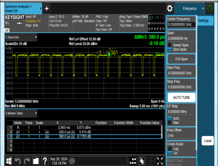
NTNV-11AC80SISO-Ant2-5530
