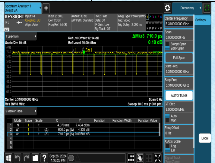
NTNV-11AC40SISO-Ant2-5310
