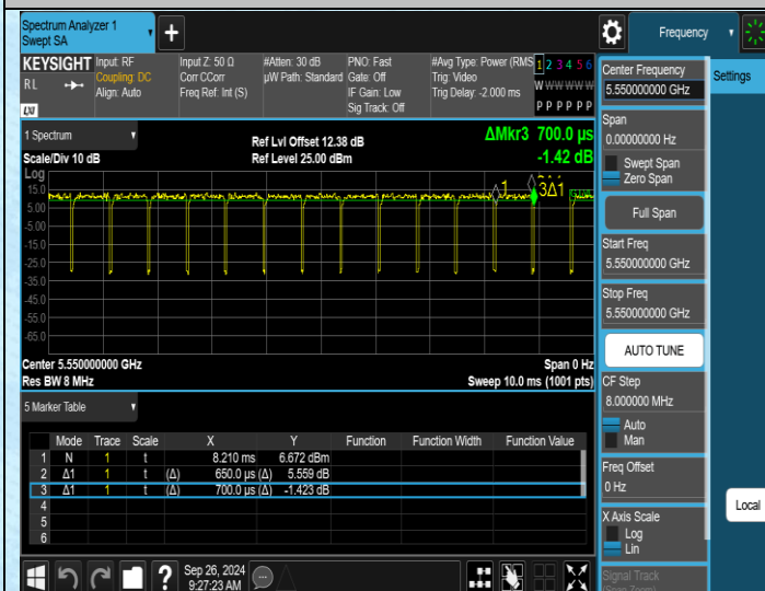
NTNV-11AC40SISO-Ant1-5550
