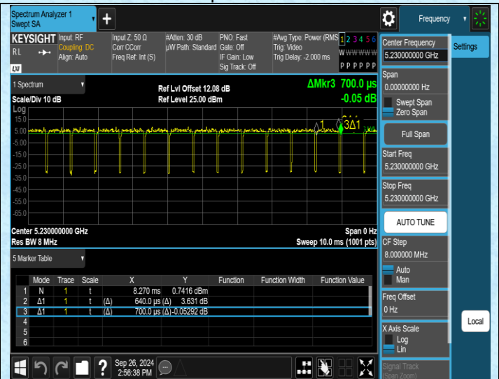
NTNV-11N40MIMO-Ant2-5230
