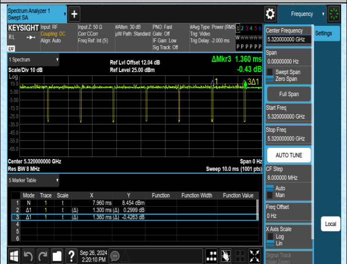
NTNV-11N20MIMO-Ant2-5320
