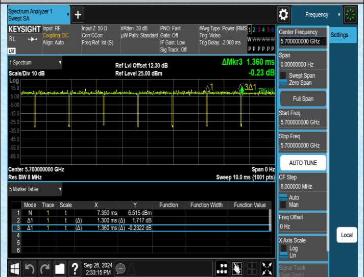
NTNV-11N20MIMO-Ant2-5700
