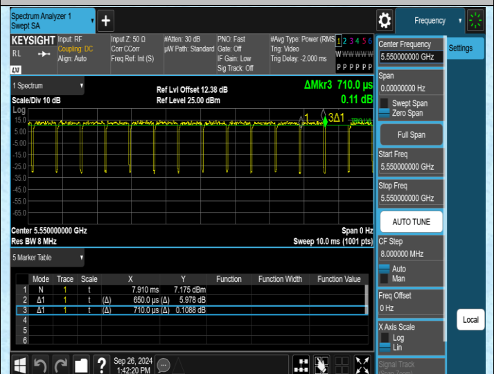
NTNV-11AC40SISO-Ant2-5550
