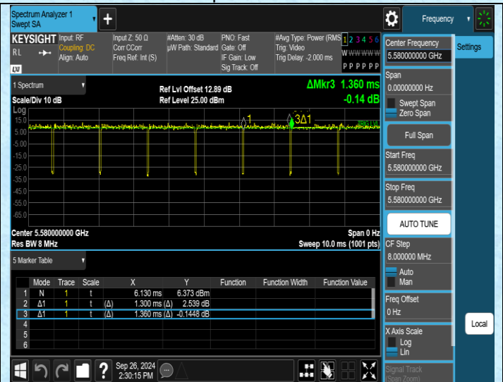
NTNV-11N20MIMO-Ant2-5580
