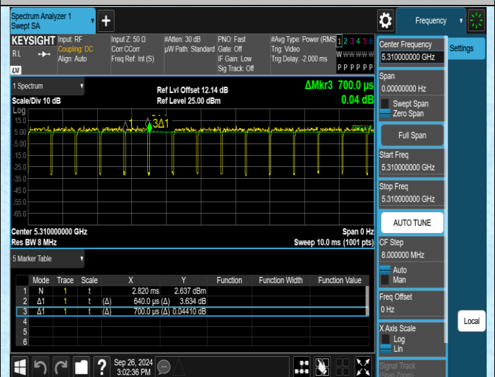
NTNV-11N40MIMO-Ant2-5310
