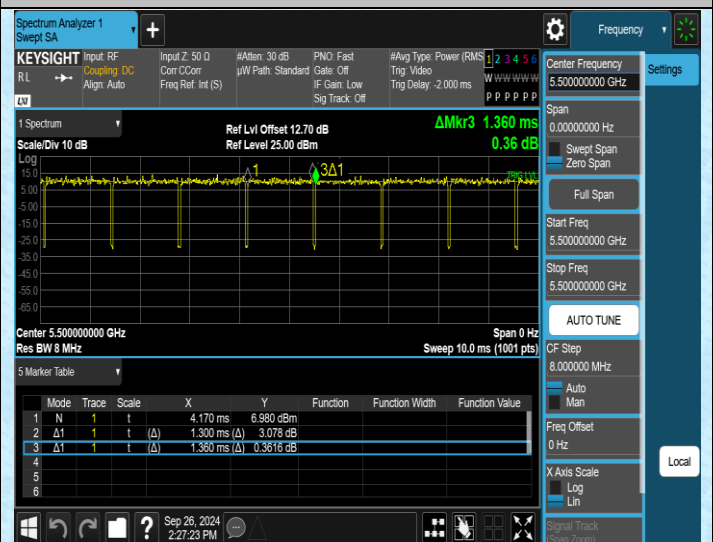
NTNV-11N20MIMO-Ant2-5500
