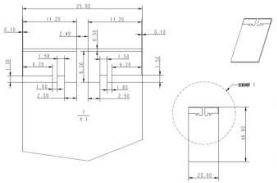
Fig 5.3 Mechanical Drawing of 5G_MODULE_FPC Module with shielding case
