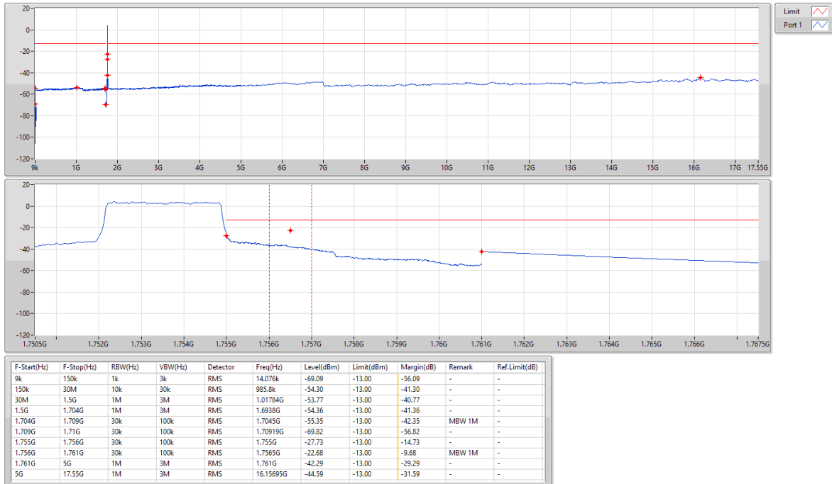
Band 4 LTE 3MHz 1TX 1753.5MHz QPSK RB 15, #RB 0
