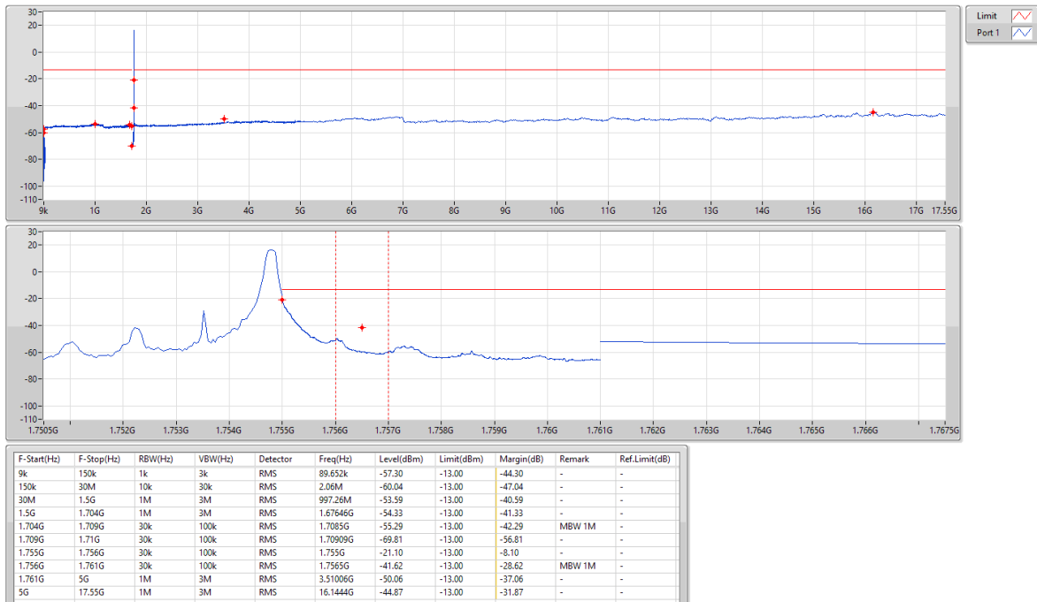
Band 4 LTE 3MHz 1TX 1753.5MHz QPSK RB 1, #RB H
