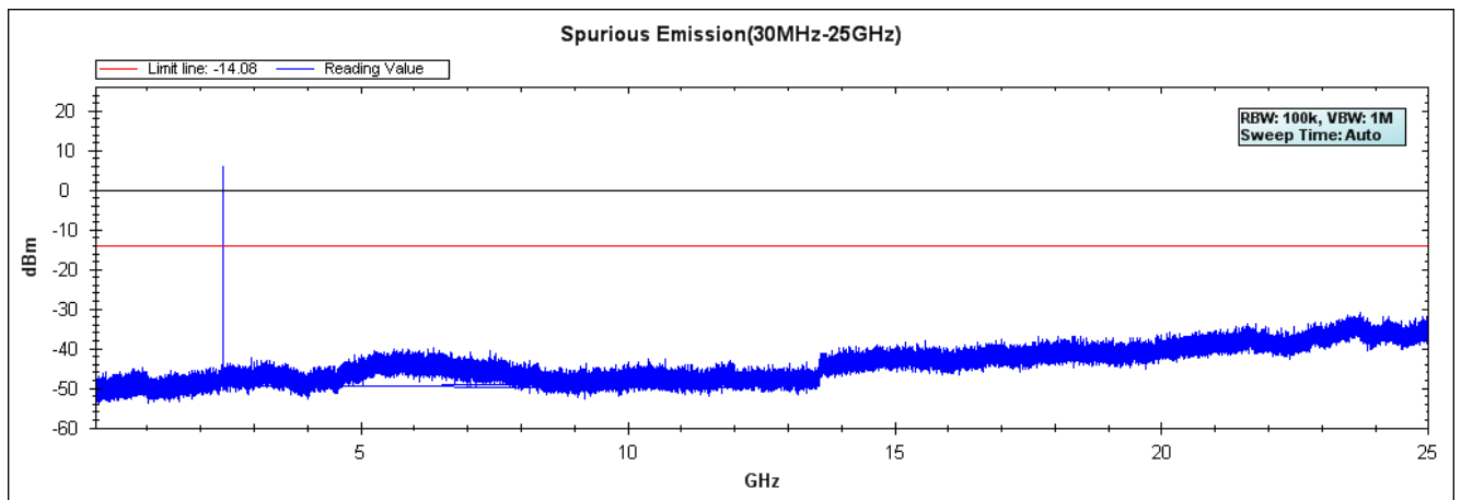
Figure Channel 39: (30M-25G)
