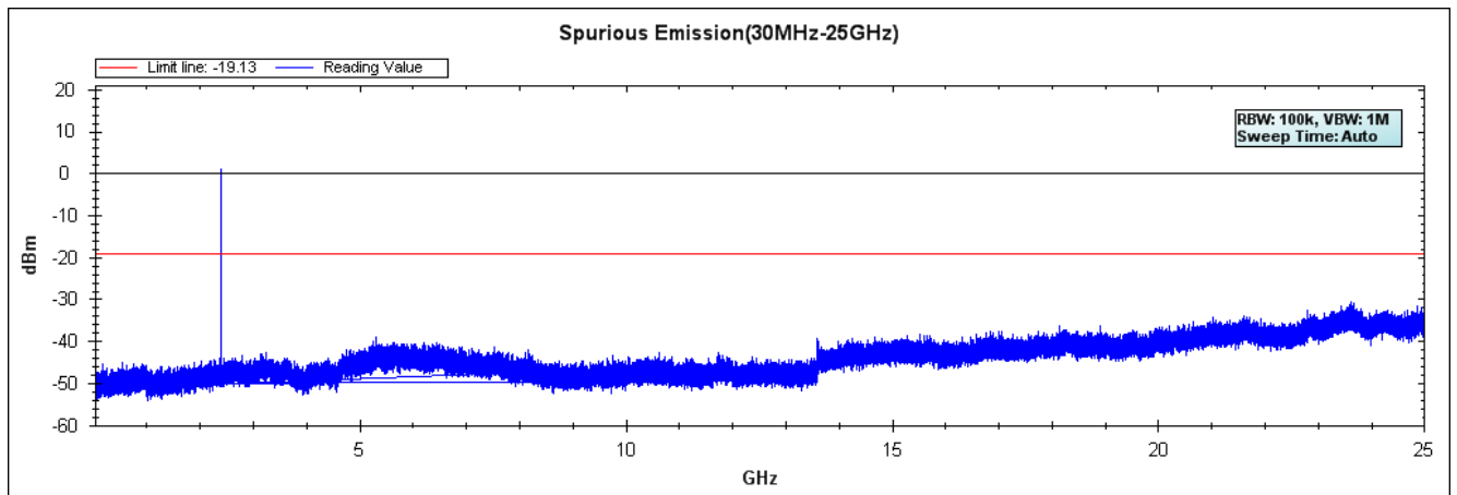
Figure Channel 00: (30M-25G)
