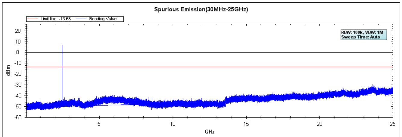
Figure Channel 78: (30M-25G)
