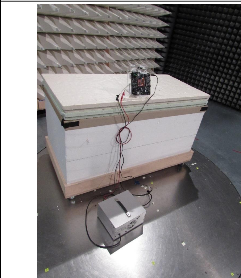
EUT Test Setup below 1 GH- Antenna 2
