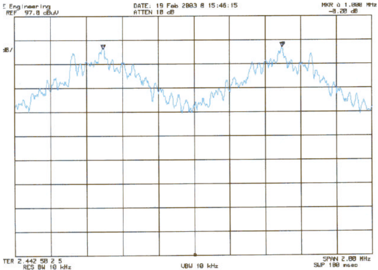
FIGURE 7 CF SEPARATION
