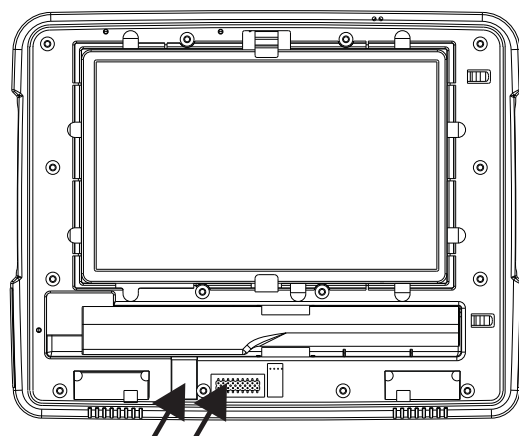
Slot on Thor VM1A Wiring Connector on Thor VM1A
