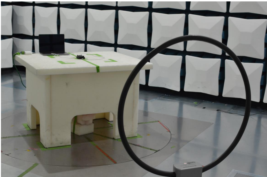
Figure 18: 9kHz-30MHz Test Setup (Front View)
