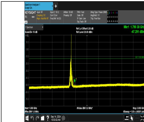
Band66_20MHz_16QAM_132072_1RB#99_1000~3000_1000~3000
