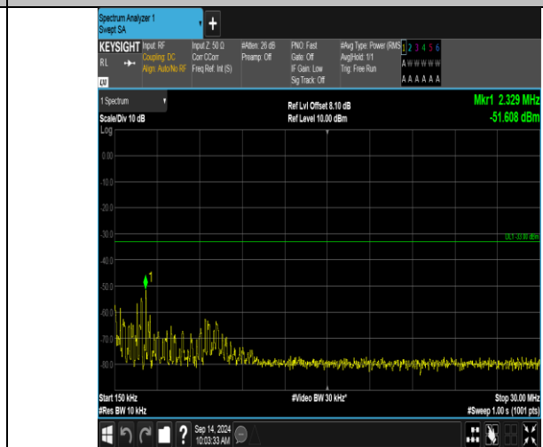
Band66_20MHz_QPSK_132072_100RB#0_0.15~30_0.15~30
