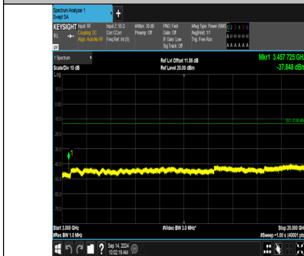
Band66_20MHz_QPSK_132072_1RB#99_3000~20000_3000~20000
