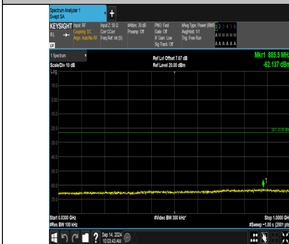
Band66_20MHz_QPSK_132072_100RB#0_30~1000_30~1000
