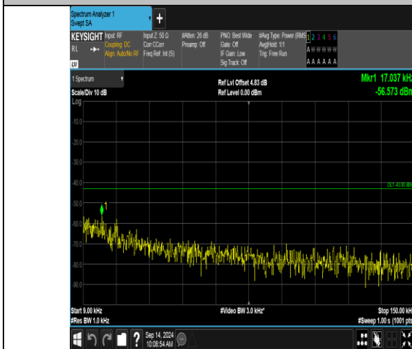
Band66_20MHz_QPSK_132322_100RB#0_0.009~0.15_0.009~0.15
