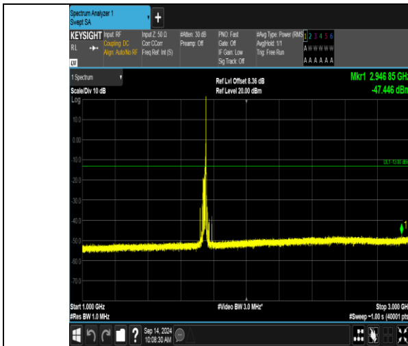
Band66_20MHz_16QAM_132322_1RB#99_1000~3000_1000~3000
