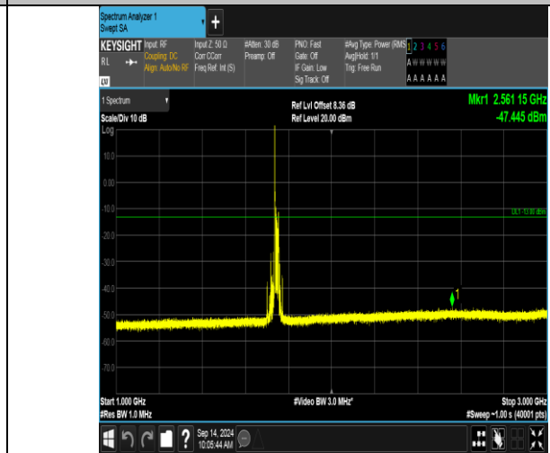
Band66_20MHz_QPSK_132322_1RB#0_1000~3000_1000~3000
