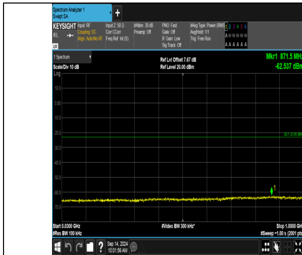
Band66_20MHz_QPSK_132072_1RB#99_30~1000_30~1000
