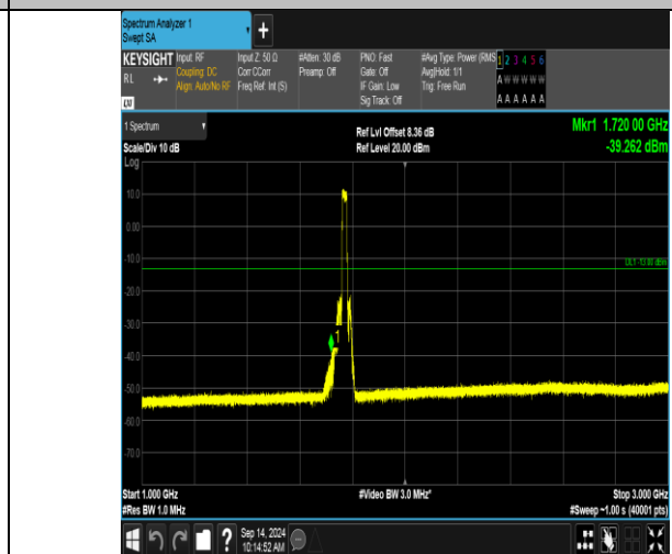
Band66_20MHz_QPSK_132572_100RB#0_1000~3000_1000~3000
