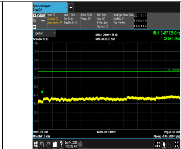
Band66_20MHz_16QAM_132072_1RB#99_3000~20000_3000~20000
