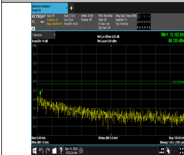
Band66_20MHz_QPSK_132072_100RB#0_0.009~0.15_0.009~0.15
