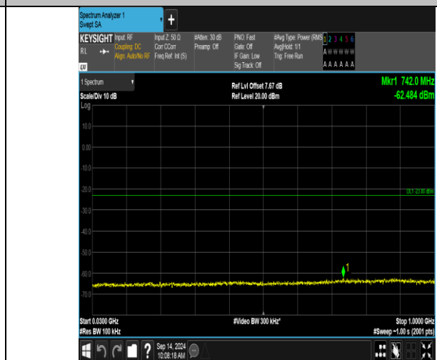
Band66_20MHz_16QAM_132322_1RB#99_30~1000_30~1000
