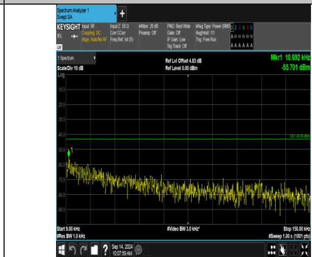
Band66_20MHz_16QAM_132322_1RB#99_0.009~0.15_0.009~0.15
