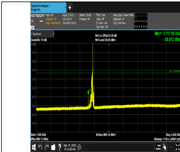
Band66_20MHz_16QAM_132572_1RB#99_1000~3000_1000~3000
