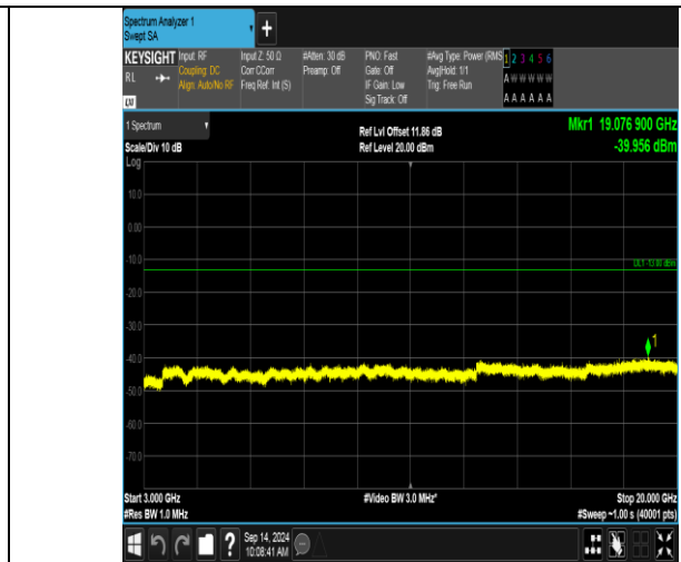
Band66_20MHz_16QAM_132322_1RB#99_3000~20000_3000~20000
