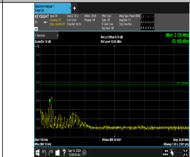
Band66_20MHz_QPSK_132322_100RB#0_0.15~30_0.15~30
