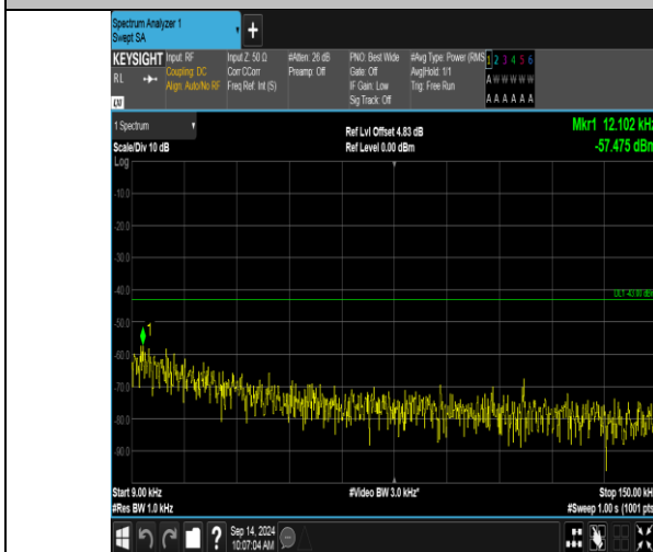
Band66_20MHz_QPSK_132322_1RB#99_0.009~0.15_0.009~0.15
