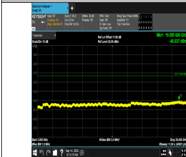
Band66_20MHz_QPSK_132572_1RB#99_3000~20000_3000~20000
