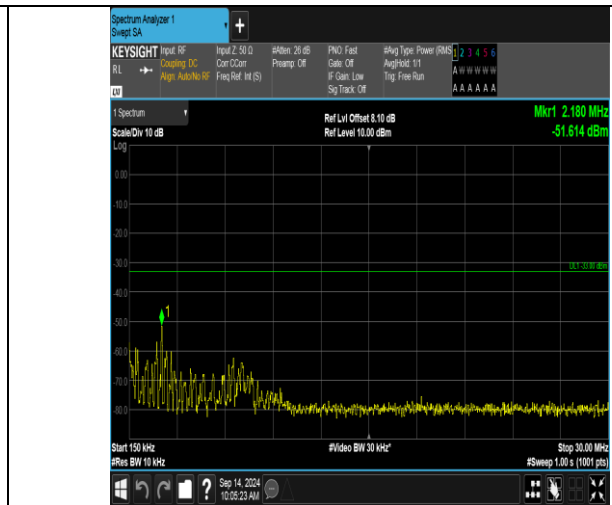
Band66_20MHz_QPSK_132322_1RB#0_0.15~30_0.15~30
