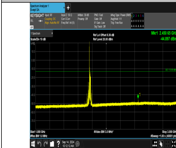
Band66_20MHz_16QAM_132572_1RB#0_1000~3000_1000~3000
