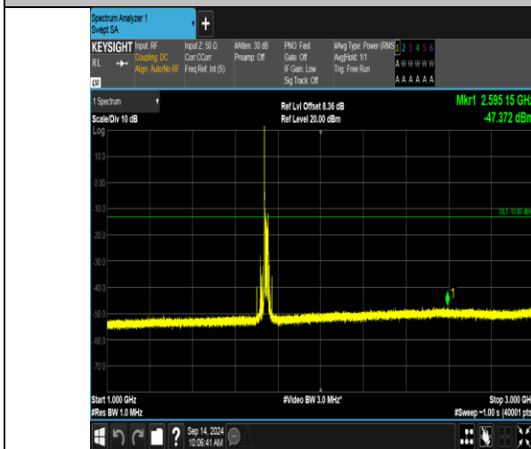
Band66_20MHz_16QAM_132322_1RB#0_1000~3000_1000~3000
