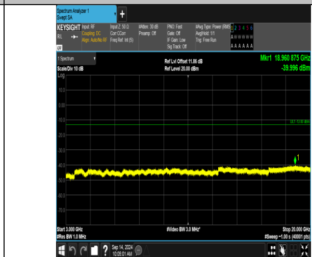
Band66_20MHz_16QAM_132072_100RB#0_3000~20000_3000~20000
