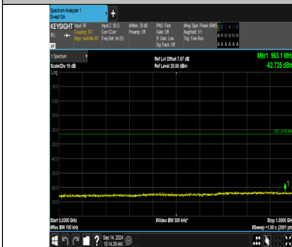
Band66_20MHz_QPSK_132572_100RB#0_30~1000_30~1000
