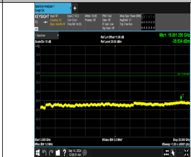
Band66_20MHz_16QAM_132322_1RB#0_3000~20000_3000~20000
