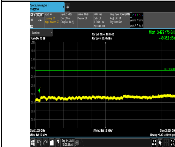
Band66_20MHz_QPSK_132322_1RB#0_3000~20000_3000~20000
