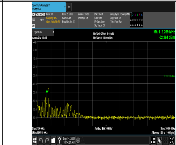
Band66_20MHz_QPSK_132572_100RB#0_0.15~30_0.15~30
