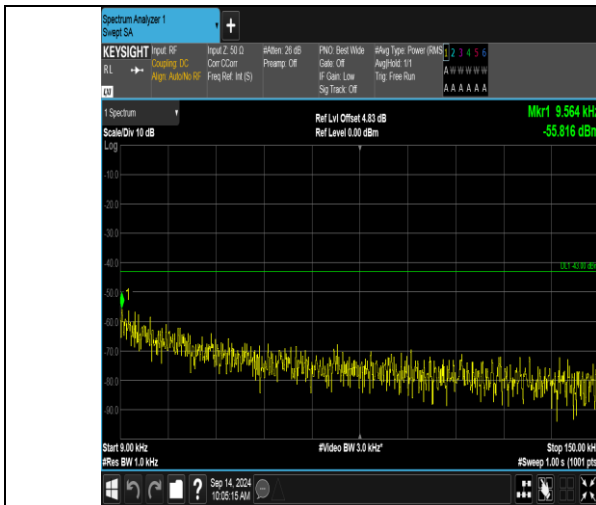
Band66_20MHz_QPSK_132322_1RB#0_0.009~0.15_0.009~0.15
