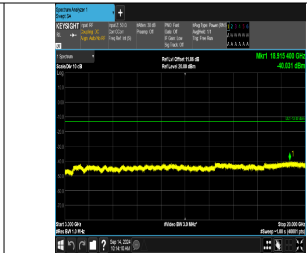
Band66_20MHz_16QAM_132572_1RB#99_3000~20000_3000~20000
