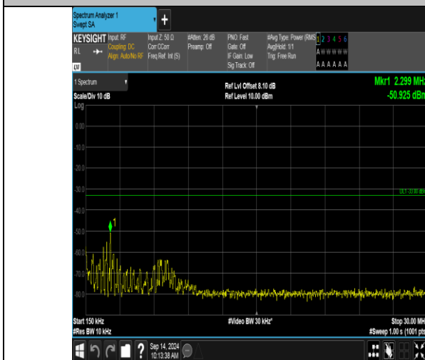
Band66_20MHz_16QAM_132572_1RB#99_0.15~30_0.15~30
