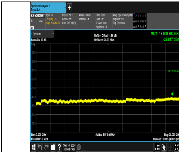
Band66_20MHz_QPSK_132072_100RB#0_3000~20000_3000~20000
