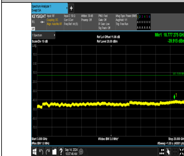
Band66_20MHz_QPSK_132322_1RB#99_3000~20000_3000~20000
