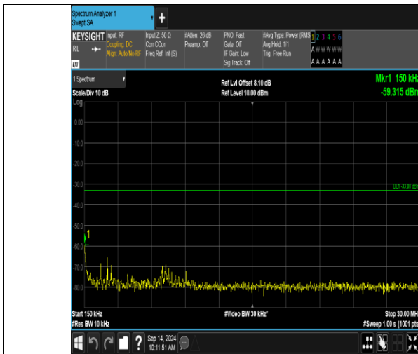
Band66_20MHz_16QAM_132572_1RB#0_0.15~30_0.15~30
