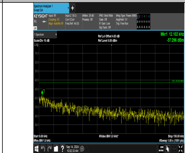
Band66_20MHz_16QAM_132072_1RB#99_0.009~0.15_0.009~0.15
