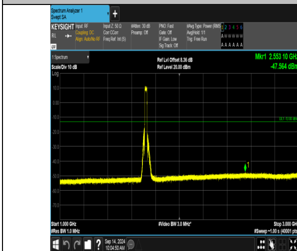
Band66_20MHz_16QAM_132072_100RB#0_1000~3000_1000~3000
