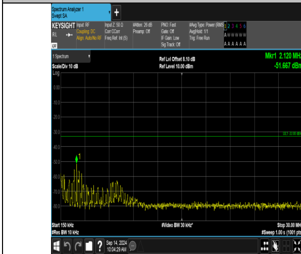
Band66_20MHz_16QAM_132072_100RB#0_0.15~30_0.15~30
