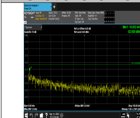
Band66_20MHz_QPSK_132572_1RB#99_0.009~0.15_0.009~0.15
