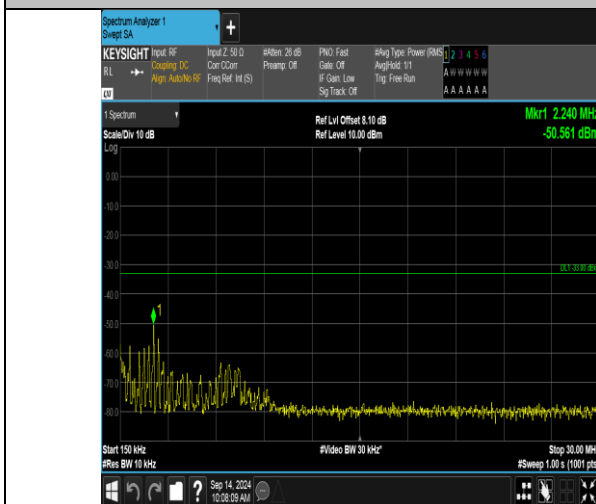
Band66_20MHz_16QAM_132322_1RB#99_0.15~30_0.15~30
