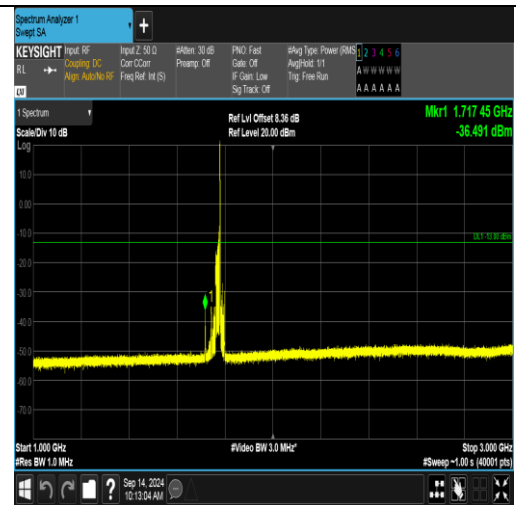
Band66_20MHz_QPSK_132572_1RB#99_1000~3000_1000~3000
