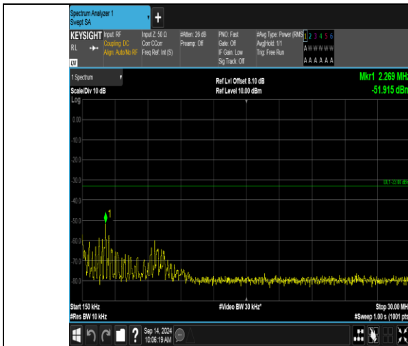
Band66_20MHz_16QAM_132322_1RB#0_0.15~30_0.15~30
