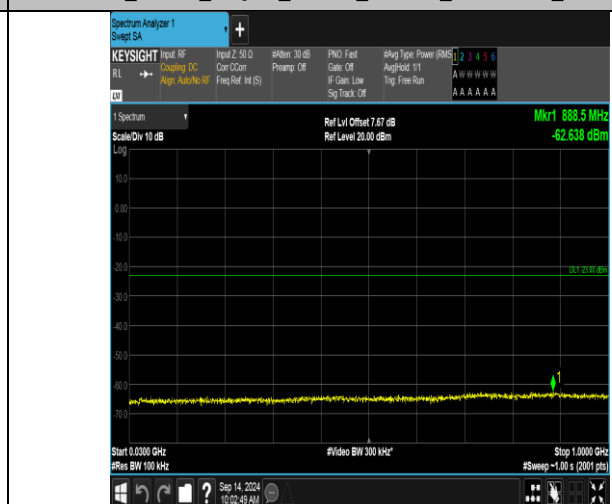
Band66_20MHz_16QAM_132072_1RB#99_30~1000_30~1000
