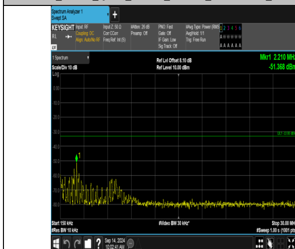
Band66_20MHz_16QAM_132072_1RB#99_0.15~30_0.15~30
