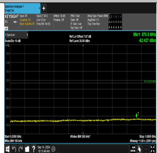
Band66_20MHz_16QAM_132572_1RB#99_30~1000_30~1000
