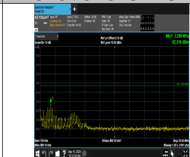
Band66_20MHz_QPSK_132572_1RB#99_0.15~30_0.15~30
