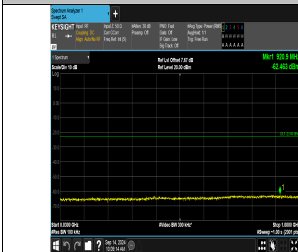
Band66_20MHz_QPSK_132322_100RB#0_30~1000_30~1000
