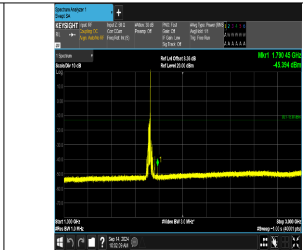
Band66_20MHz_QPSK_132072_1RB#99_1000~3000_1000~3000
