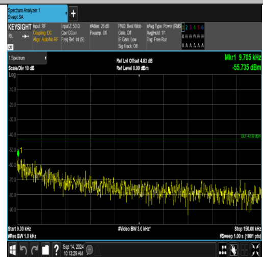
Band66_20MHz_16QAM_132572_1RB#99_0.009~0.15_0.009~0.15
