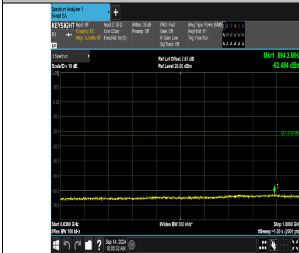
Band66_20MHz_QPSK_132322_1RB#0_30~1000_30~1000
