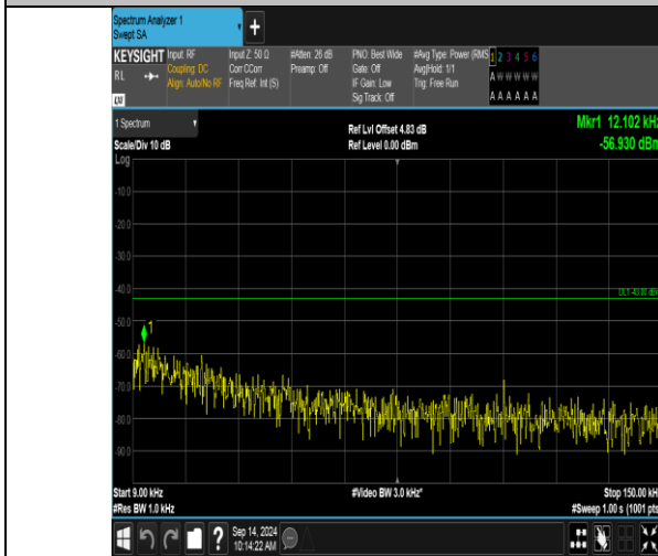
Band66_20MHz_QPSK_132572_100RB#0_0.009~0.15_0.009~0.15
