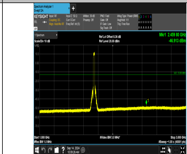
Band66_20MHz_QPSK_132322_100RB#0_1000~3000_1000~3000
