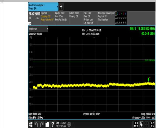
Band66_20MHz_16QAM_132572_1RB#0_3000~20000_3000~20000
