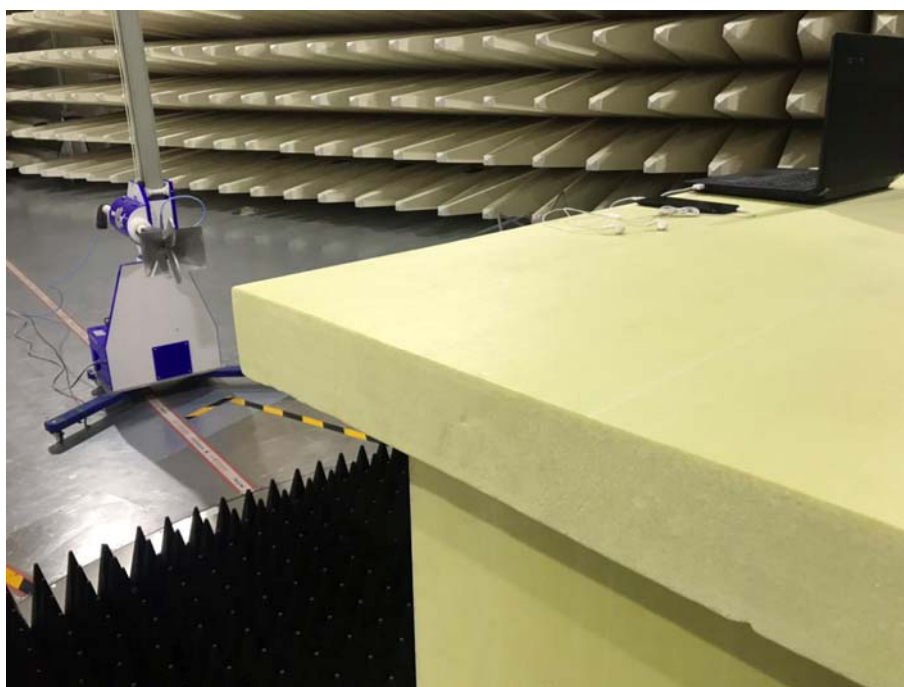
Above 1GHz Radiated Emissions Test Setup (with laptop)
