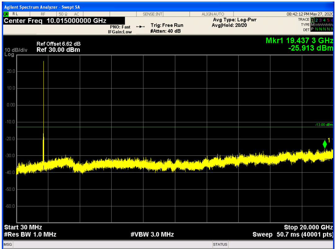
LTE Band4 QAM16 BW=15MHz Channel=20325 RB Size=75 Position=#0
