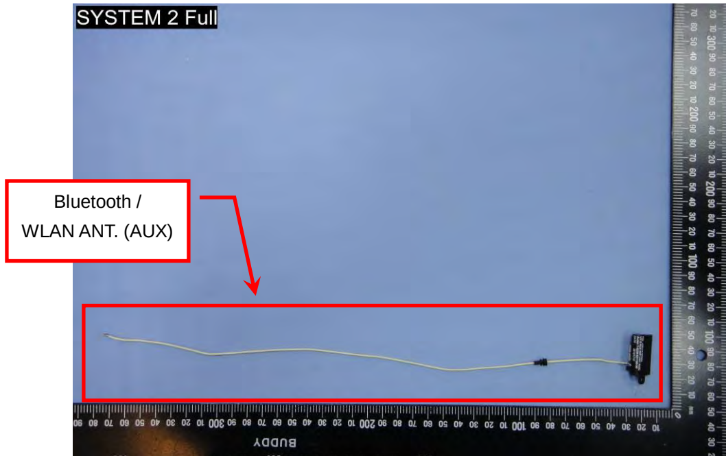
EUT Photo (22)
