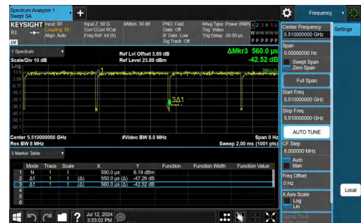
NTNV-11AX40SISO-Ant1-5670
