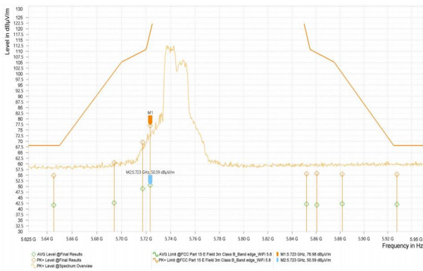
Wi-Fi 5G_11AX20_5745_52Tone_RU37
