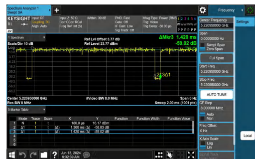
NTNV-11AX20SISO-Ant1-5220-106Tone-RU53
