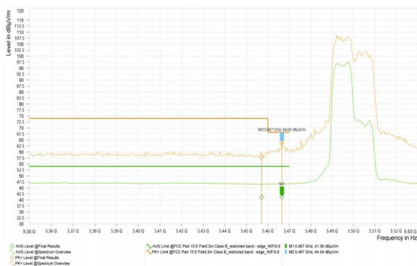
Wi-Fi 5G_11AX20_5500_52Tone_RU37
