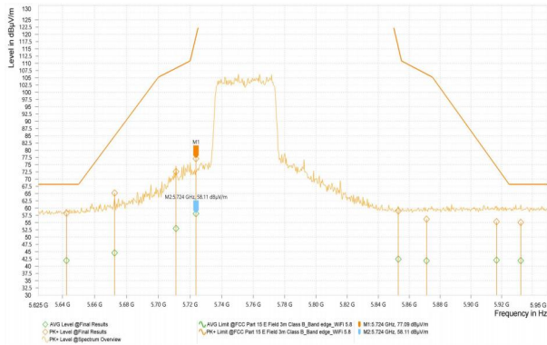
Wi-Fi 5G_11AX40_5755
