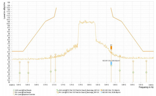
Wi-Fi 5G_11AX40_5795
