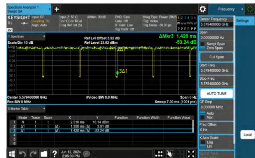
NTNV-11AX20SISO-Ant1-5580-106Tone-RU53
