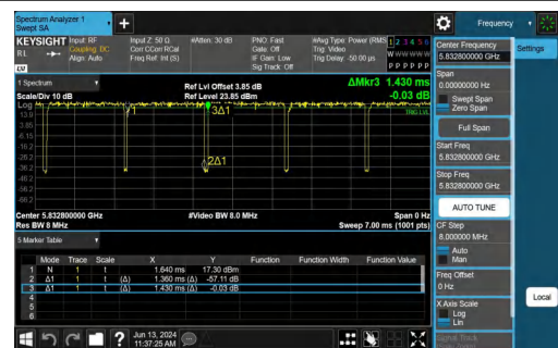
NTNV-11AX20SISO-Ant1-5825-106Tone-RU54
