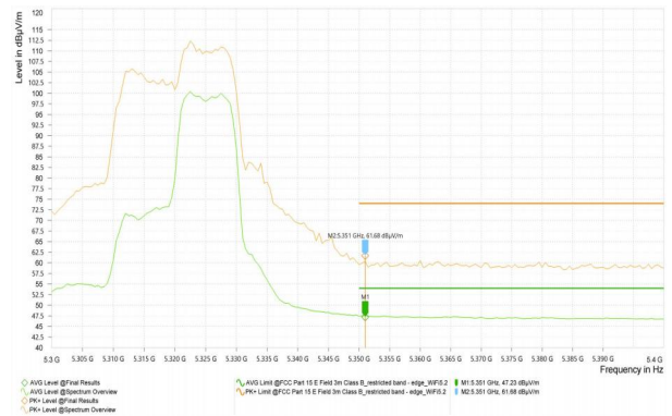
Wi-Fi 5G_11AX20_5320_52Tone_RU40
