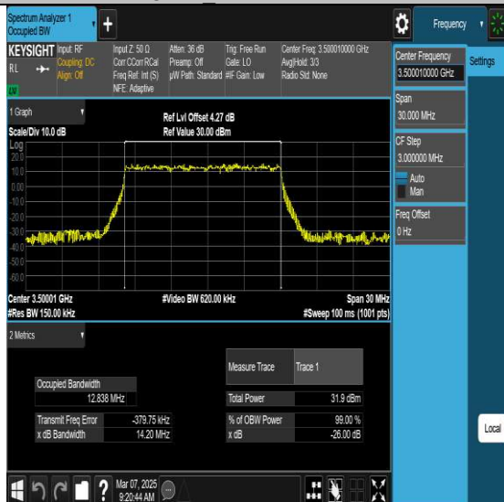
NTNV-N77-3450-3550-PC2-30-15-M-DFT-QPSK-Outer Full-Ant1-PASS
