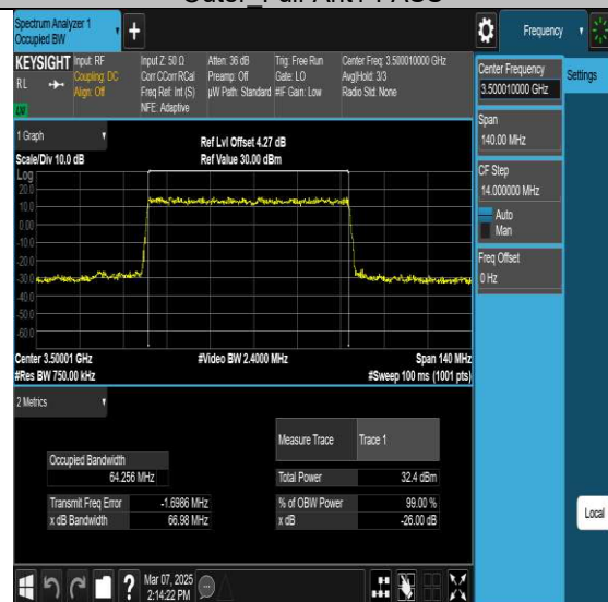
NTNV-N77-3450-3550-PC2-30-70-M-DFT-QPSK-Outer_Full-
