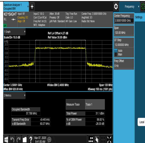
NTNV-N77-3450-3550-PC2-30-60-M-DFT-16QAM-Outer_Full-Ant1-PASS
