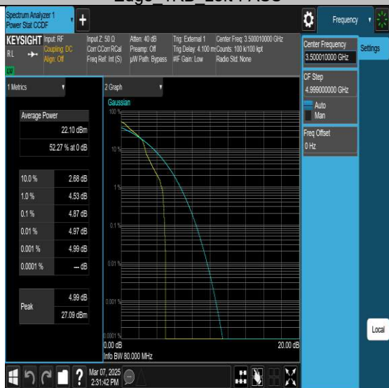
NTNV-N77-3450-3550-PC2-30-80-M-DFT-QPSK
