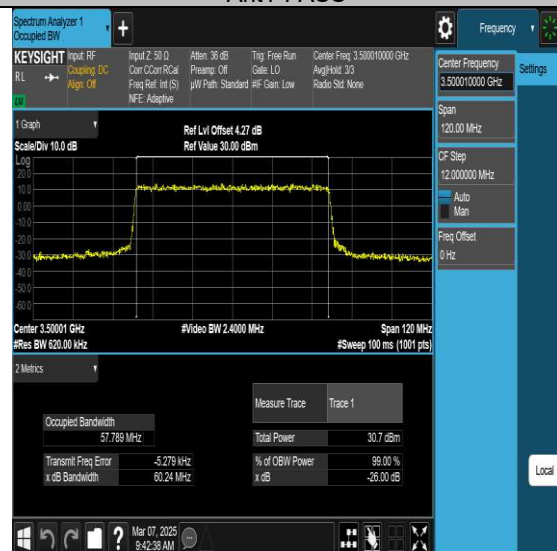
NTNV-N77-3450-3550-PC2-30-60-M-DFT-256QAM-Outer_Full-Ant1-PASS
