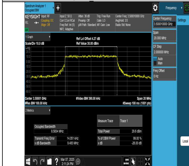
NTNV-N77-3450-3550-PC2-30-10-M-DFT-16QAM-Outer_Full-Ant1-PASS
