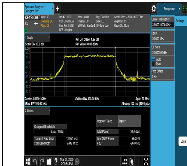
NTNV-N77-3450-3550-PC2-30-10-M-DFT-PI2BPSK-Outer_Full-Ant1-PASS
