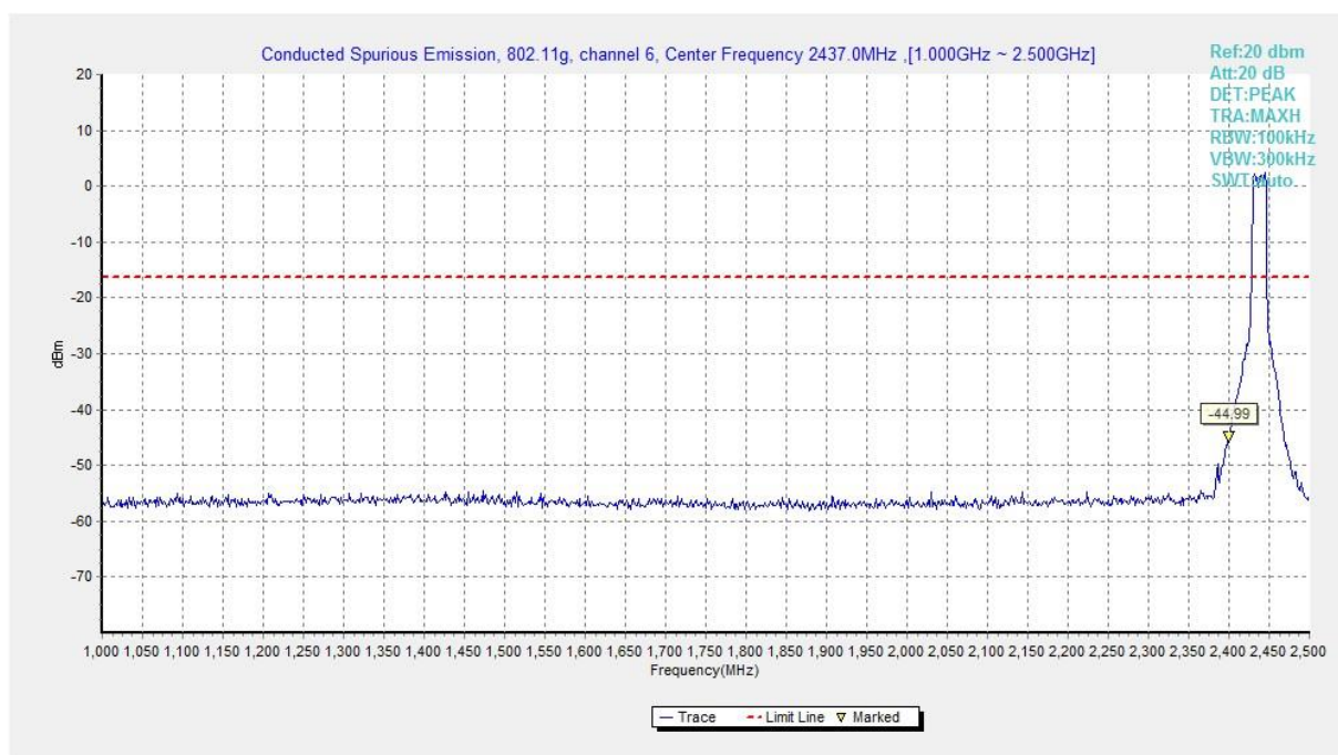
Fig.B.6.1.35 Transmitter Spurious Emission - Conducted (802.11g, Ch6, 1 GHz-2.5 GHz)
