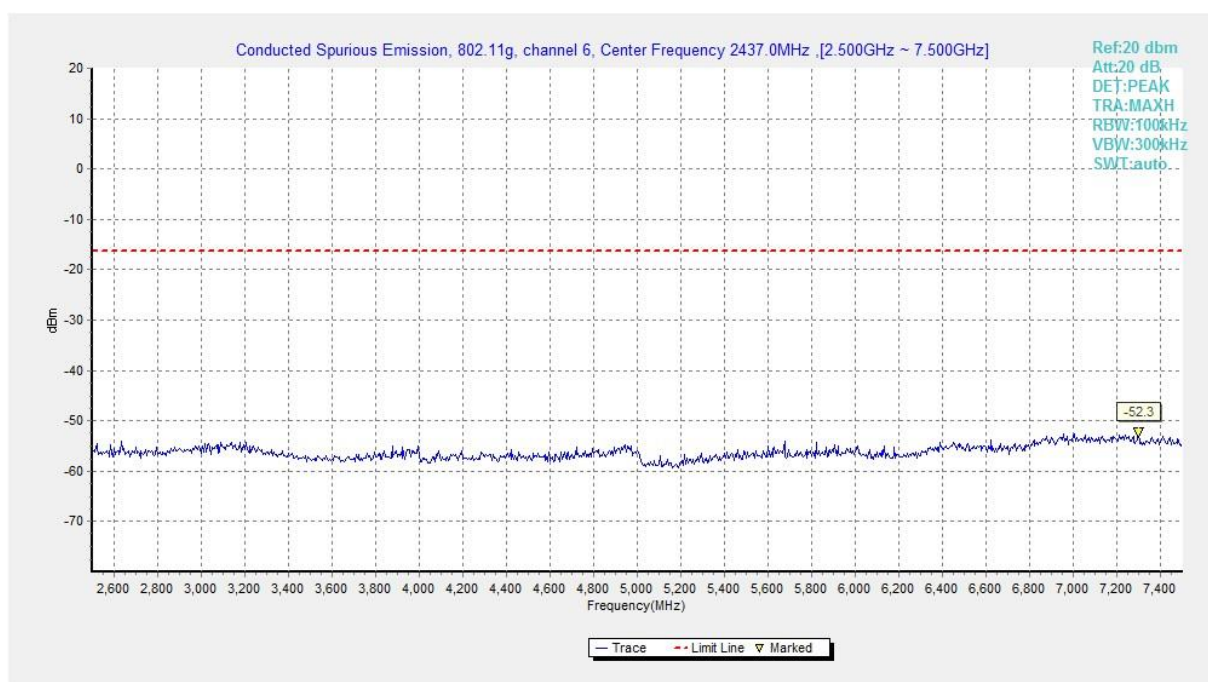
Fig.B.6.1.36 Transmitter Spurious Emission - Conducted (802.11g, Ch6, 2.5 GHz-7.5 GHz)
