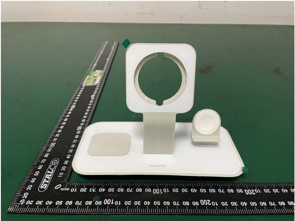
External Photos M/N: WRLS-BYO-MS-WCH
