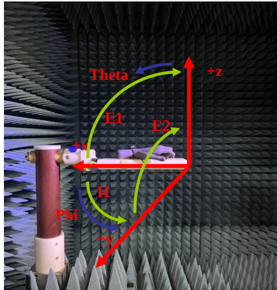
Figure 4: Geometry for SM-R861/R866 for Radiation patterns.
