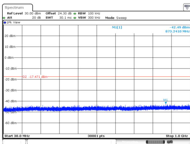
CSE Plot on Low Ch between 30MHz ~ 1 GHz
