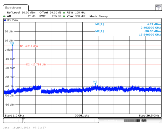
CSE Plot on Low Ch between 1 GHz ~ 26.5 GHz
