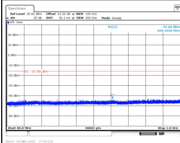
CSE Plot on Low Ch between 30MHz ~ 1 GHz
