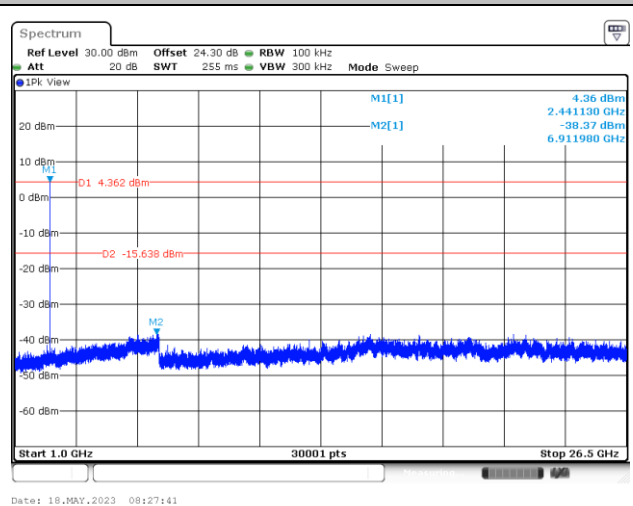
CSE Plot on Mid. Ch between 1 GHz ~ 26.5 GHz
