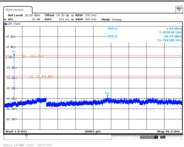
CSE Plot on Low Ch between 1 GHz ~ 26.5 GHz
