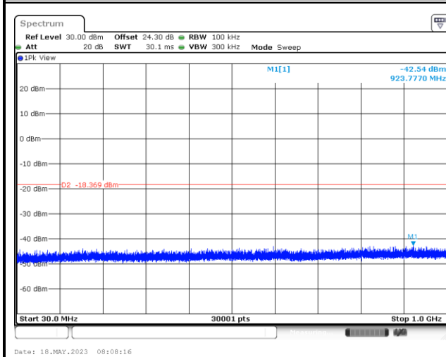
CSE Plot on Low Ch between 30MHz ~ 1 GHz
