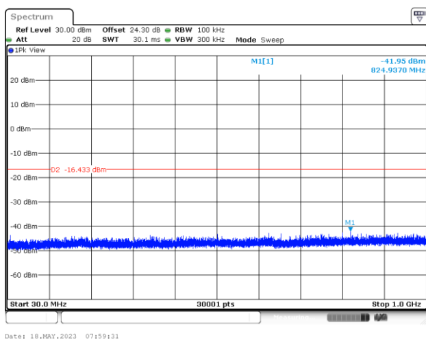
CSE Plot on Mid. Ch between 30MHz ~ 1 GHz
