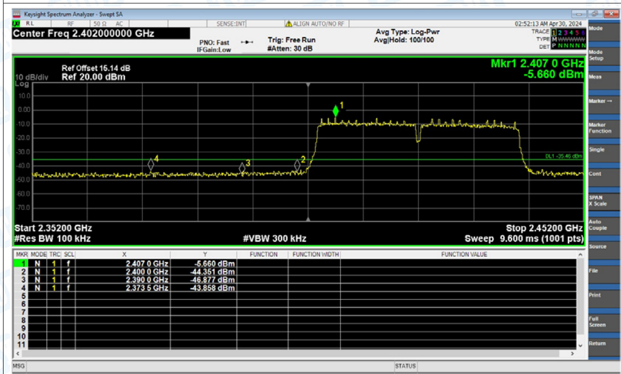
Band Edge NVNT n(HT40) 2422MHz Ant2 Emission
