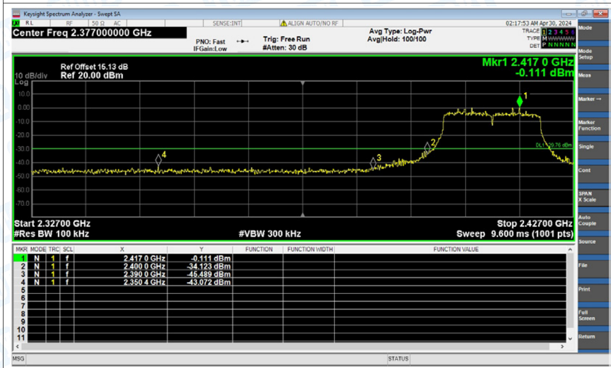
Band Edge NVNT n(HT20) 2412MHz Ant2 Emission
