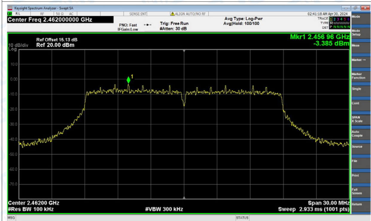
Band Edge NVNT n(HT20) 2462MHz Ant2 Emission
