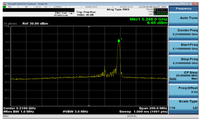
Plot 7-155. PSD Antenna 5T (80MHz BW 11ax Index 36 – RU26 – Ch.42)
