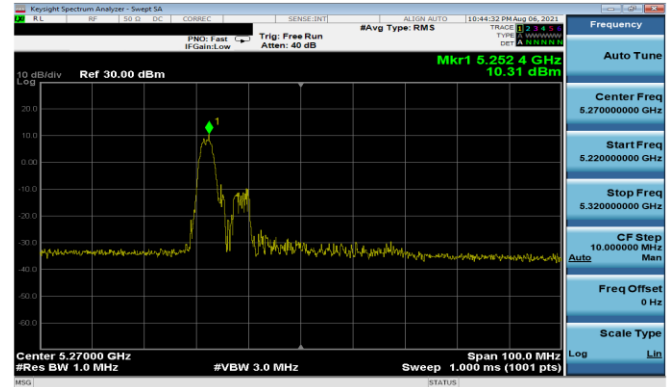
Plot 7-161. PSD Antenna 5T (40MHz BW 11ax Index 0 - RU26 - Ch.54)
