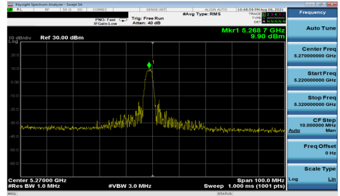
Plot 7-162. PSD Antenna 5T (40MHz BW 11ax Index 8 - RU26 - Ch.54)
