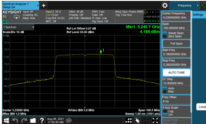
Plot 7-152. PSD Antenna 5T (40MHz BW 11ax – RU484 – Ch.46)
