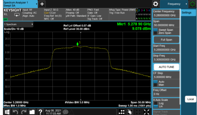
Plot 7-160. PSD Antenna 5T (20MHz BW 11ax- RU242 - Ch.56)
