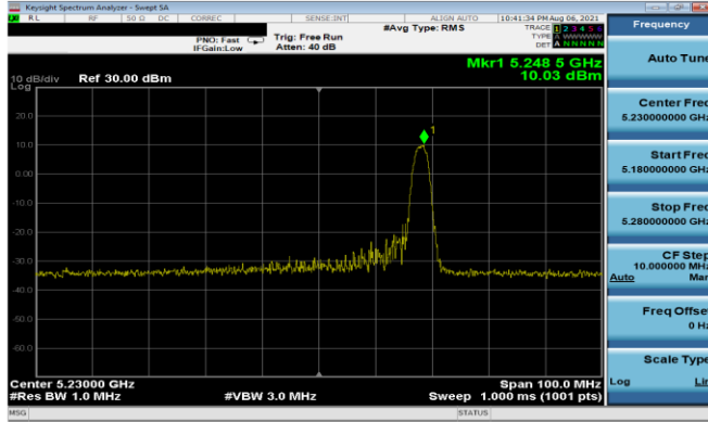
Plot 7-151. PSD Antenna 5T (40MHz BW 11ax Index 17 – RU26 – Ch.46)
