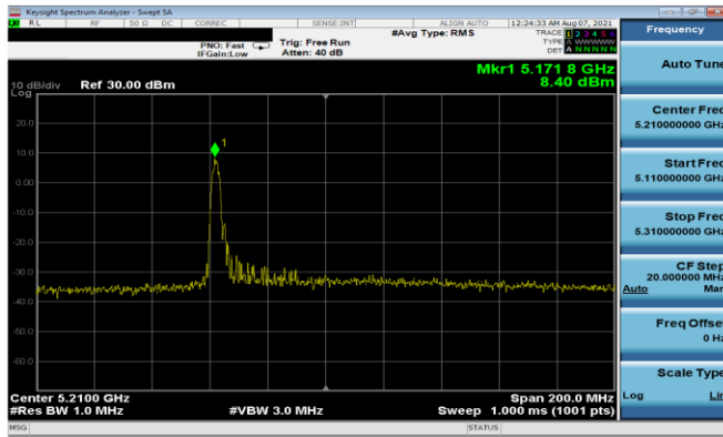
Plot 7-153. PSD Antenna 5T (80MHz BW 11ax Index 0 – RU26 – Ch.42)
