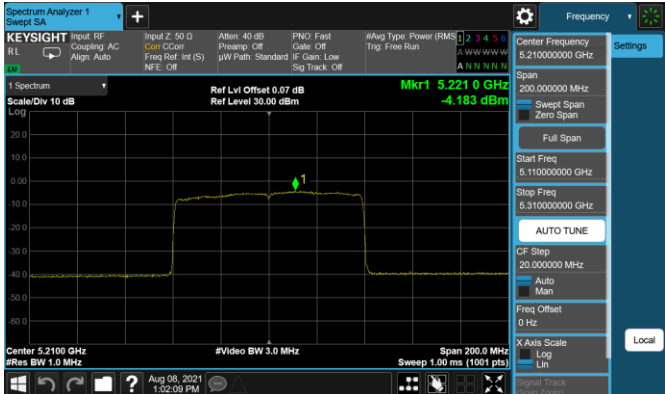
Plot 7-156. PSD Antenna 5T (80MHz BW 11ax – RU996 – Ch.42)
