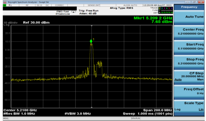
Plot 7-154. PSD Antenna 5T (80MHz BW 11ax Index 18 – RU26 – Ch.42)
