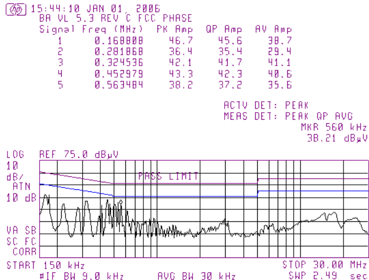
Plot 1. Subscriber Unit Conducted emissions measurement result on 120 VAC power line: phase
