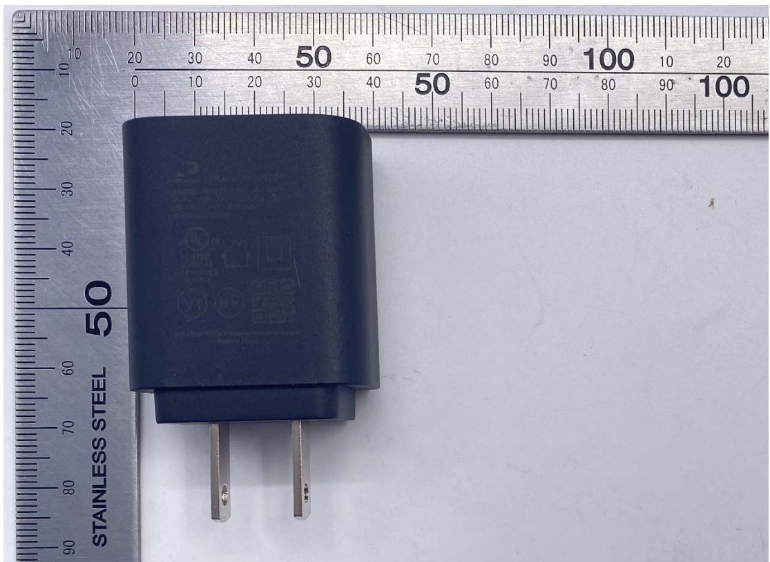
Charger View (Model: RD0502000-USBA-87MGmade by Ruide)
