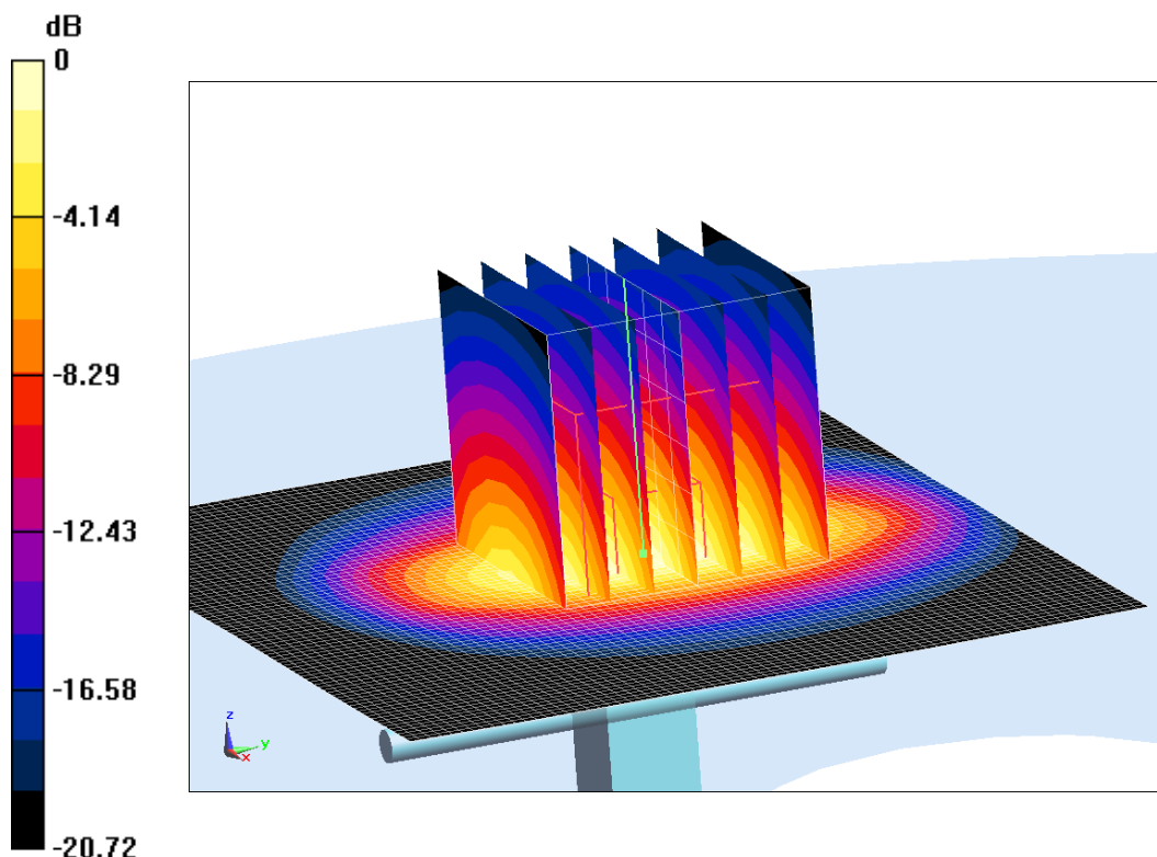
Fig.B.8 validation 2300 MHz 250mW
