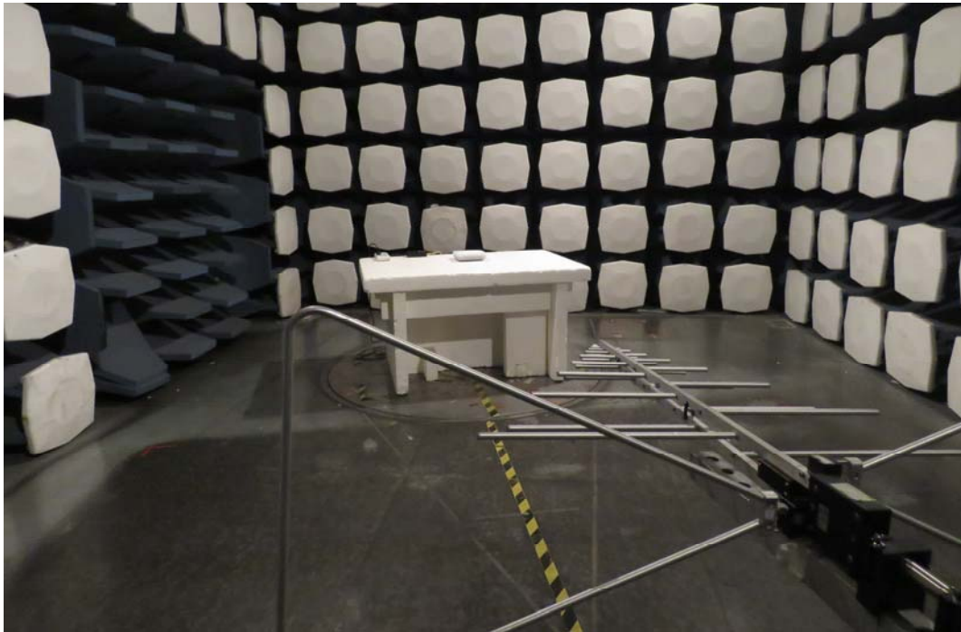
FCC Part15E Radiated Emission Test Setup
