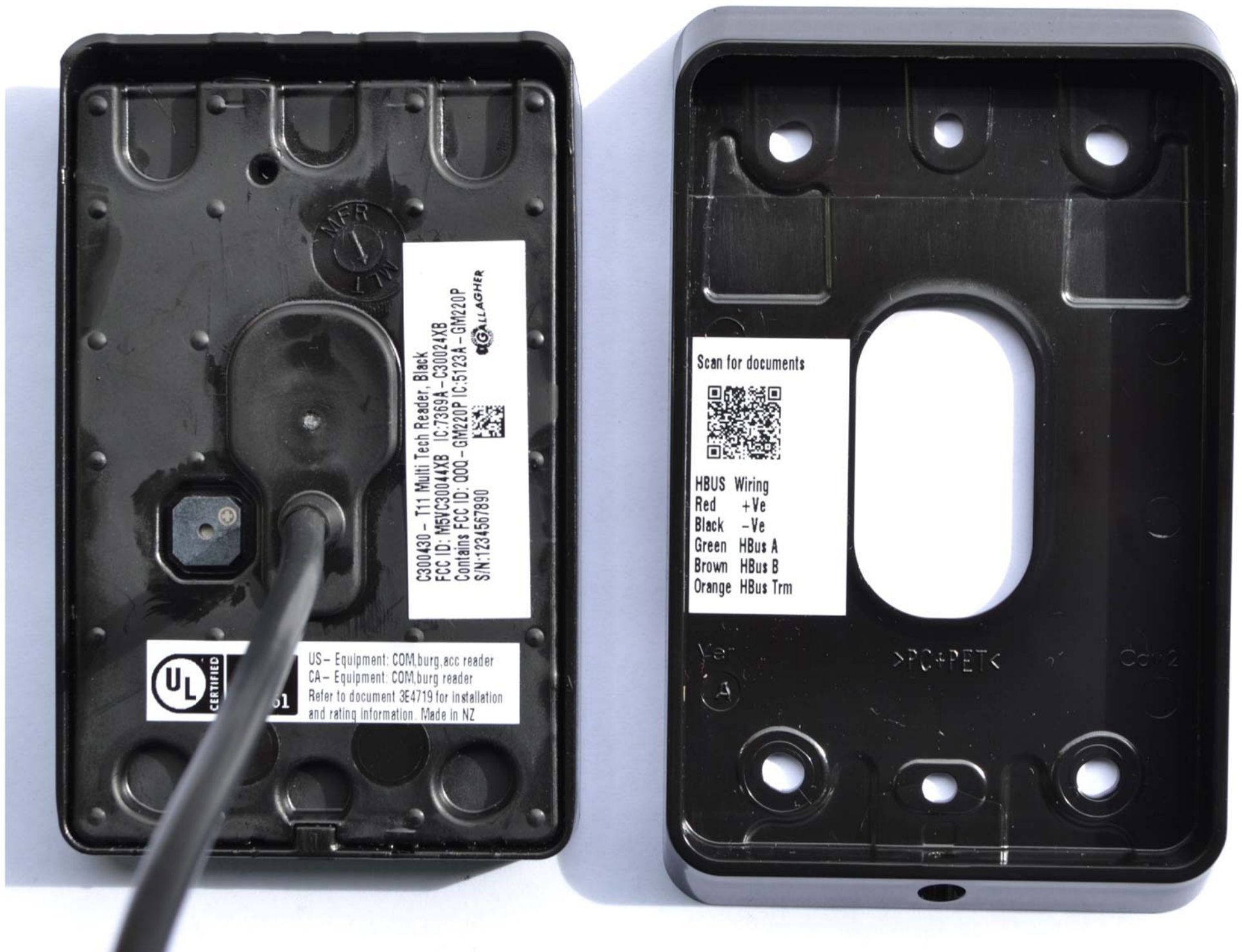
T11 Mifare/ Multi Tech/ SMB T11 - Potted Assembly
