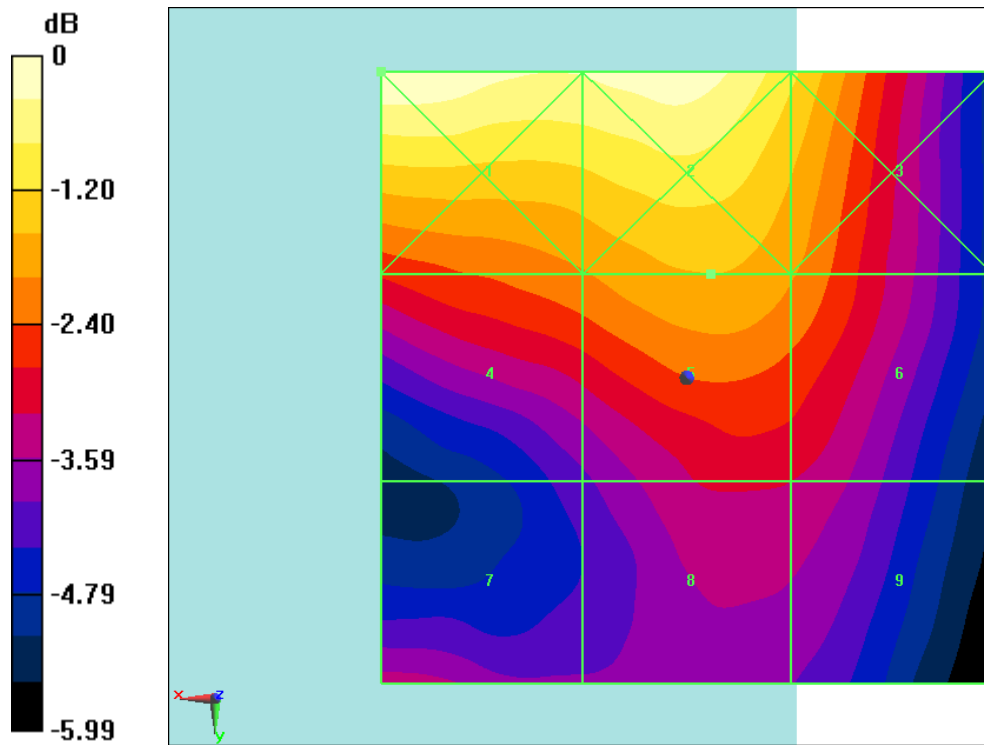
Fig B.4 HAC RF E-Field WiFi2.4G 11g
