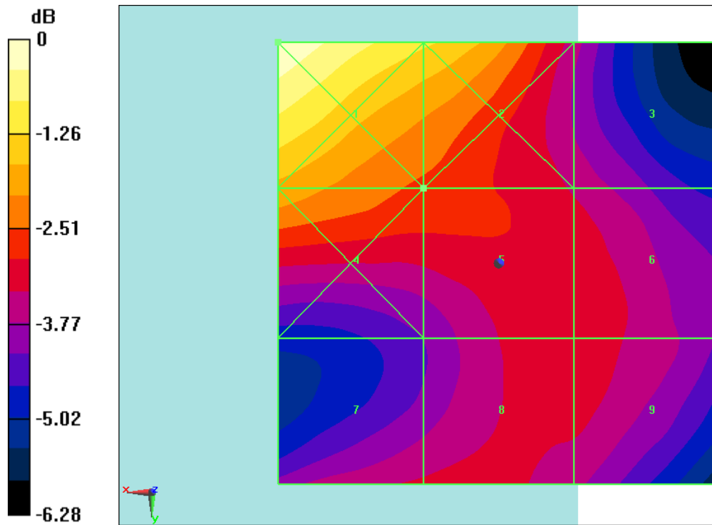
Fig B.3 HAC RF E-Field LTE Band41 QPSK CH40800
