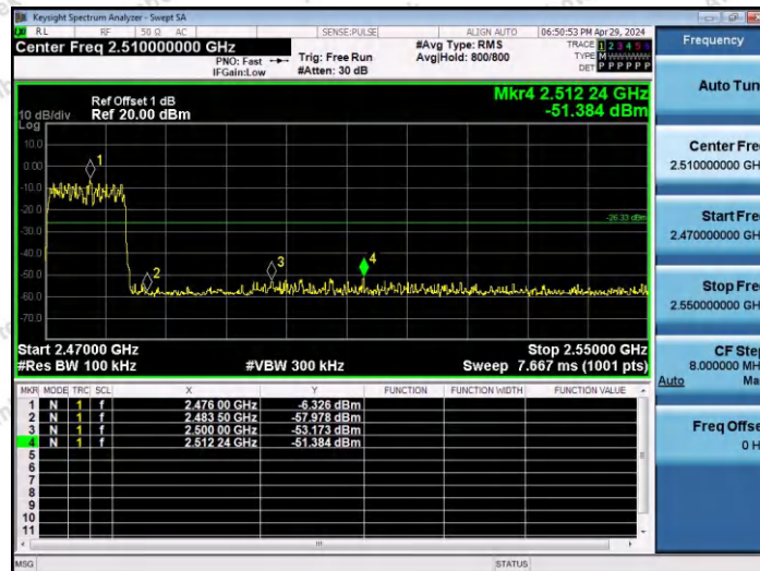
2DH5-Ant1-Hop_2480-PASS
