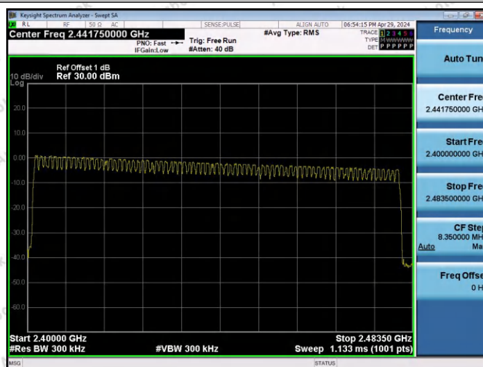
2DH5-Ant1-Hop-PASS
