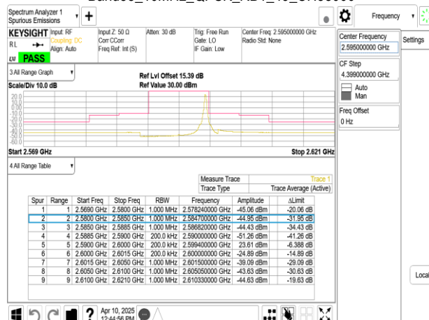
Band38_10MHz_QPSK_RB1_49_CH38000
