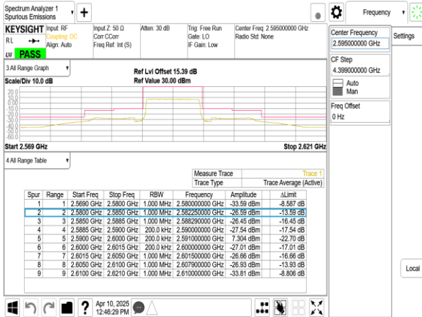
Band38_10MHz_QPSK_RB1_0_CH38200
