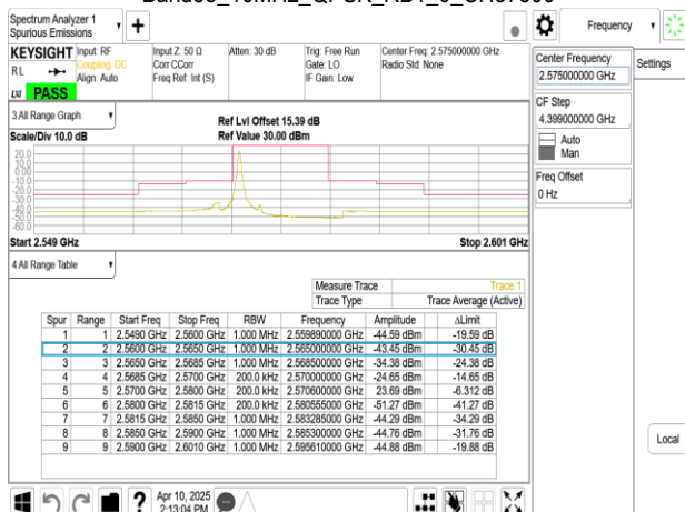
Band38_10MHz_QPSK_RB1_49_CH37800
