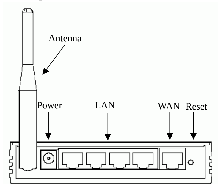
Figure 2 – Wireless 802.11g Broadband Router Rear Panel
