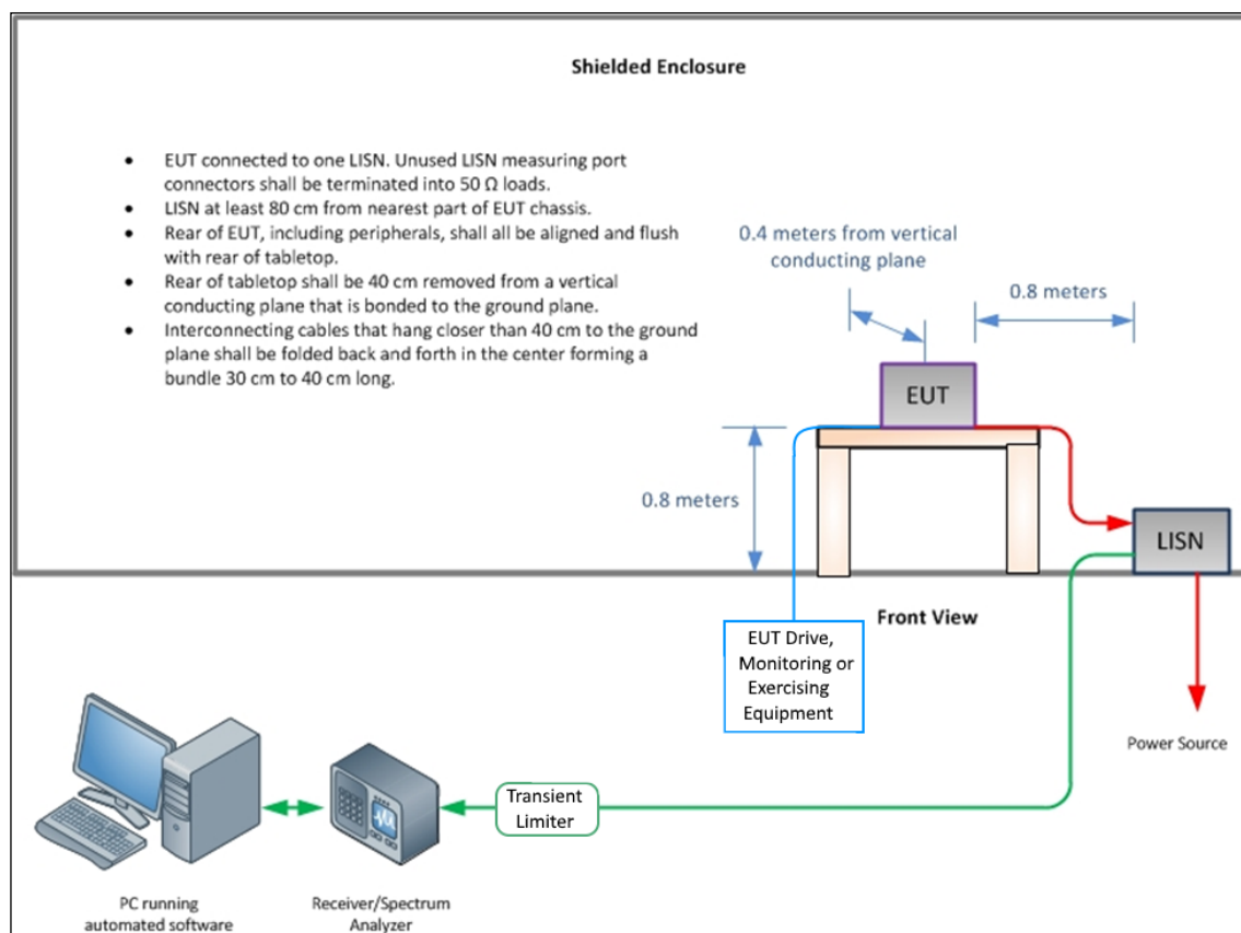
Figure 1 - Conducted Disturbance
