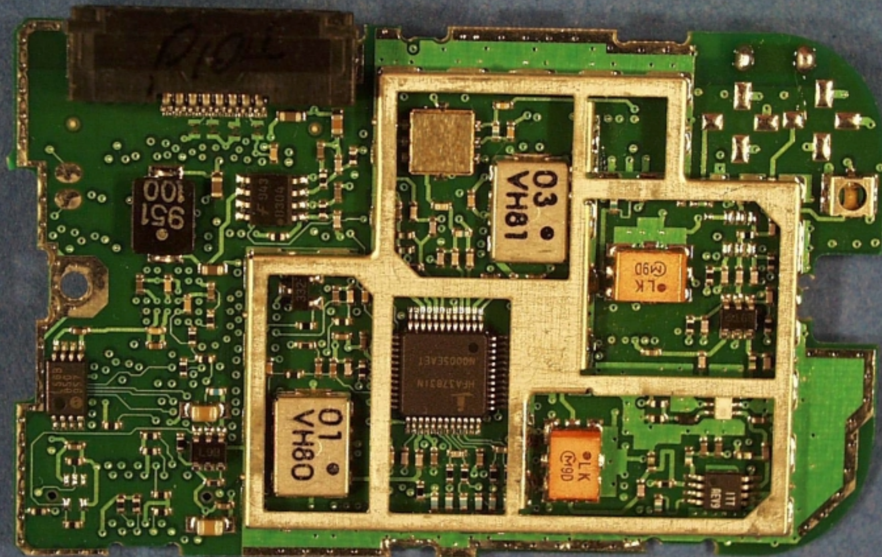
DM4046 RF Side Cover Removed NP4046 Configuraton
