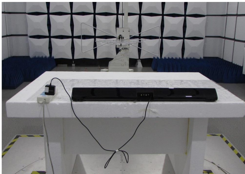
Radiated Emission Below 1GHz
