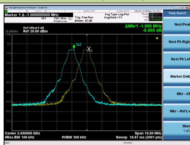
Channel 78 (2480MHz)
