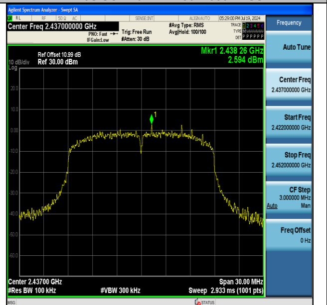
11N20SISO-Ant1-2437-0~Reference-PASS
