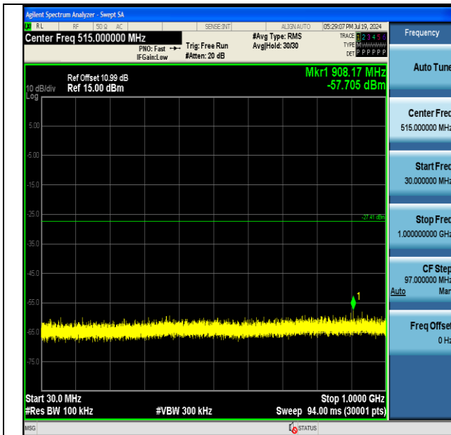
11N20SISO-Ant1-2437-30~1000-PASS
