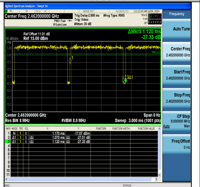
NTNV-11AX20SISO-Ant1-2462
