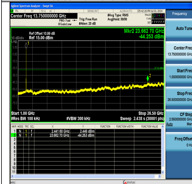
11AX20SISO-Ant1-2437-1000~26500-PASS
