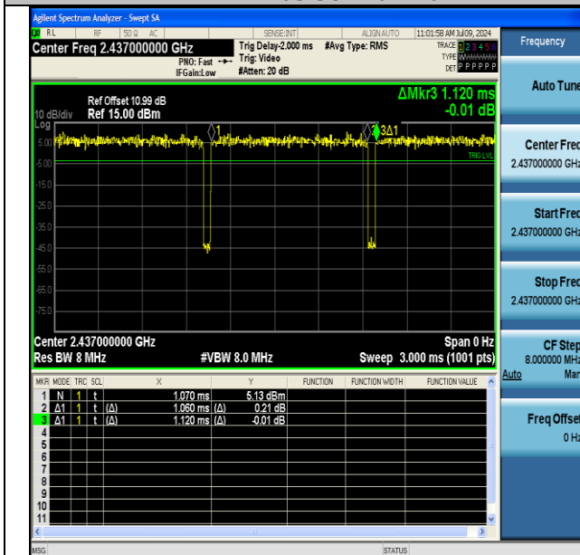
NTNV-11AX20SISO-Ant1-2437
