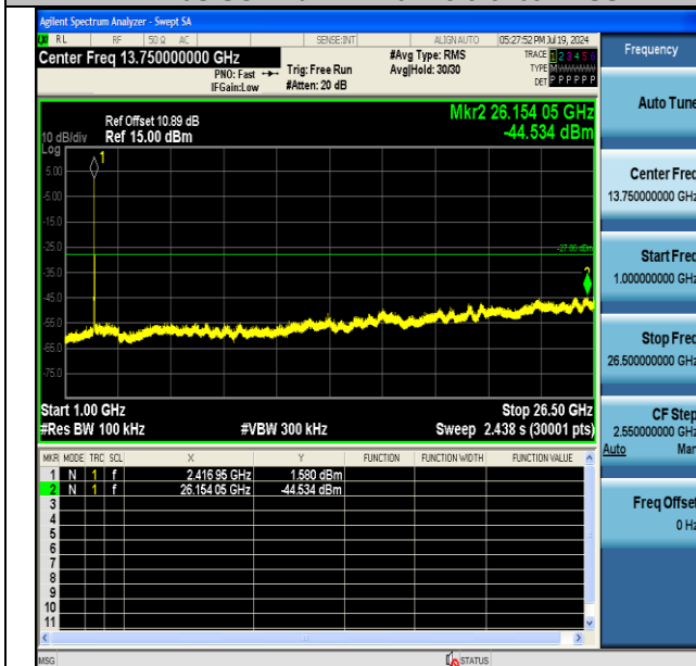
11N20SISO-Ant1-2412-1000~26500-PASS
