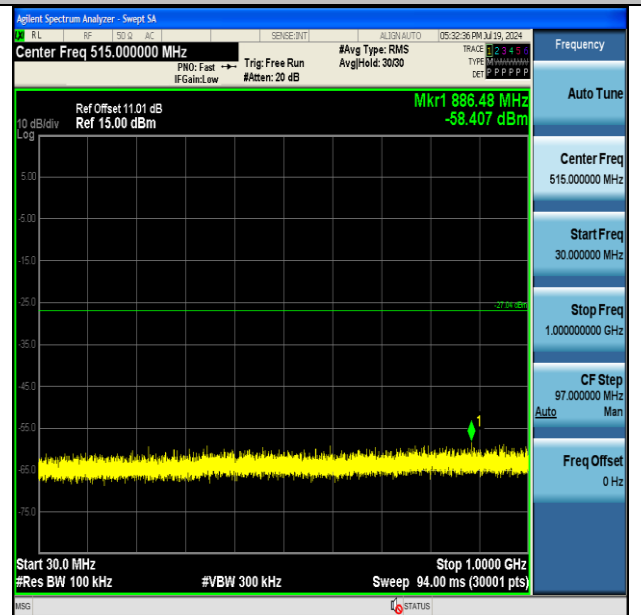
11N20SISO-Ant1-2462-30~1000-PASS
