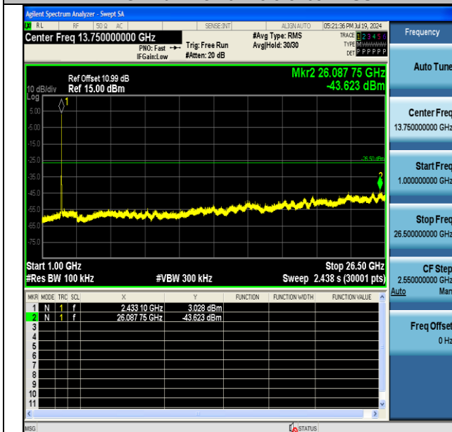
11G-Ant1-2437-1000~26500-PASS
