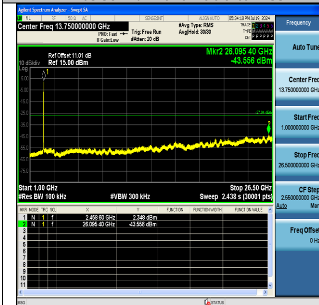
11N20SISO-Ant1-2462-1000~26500-PASS
