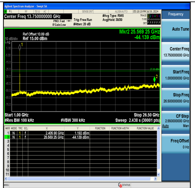
11G-Ant1-2412-1000~26500-PASS
