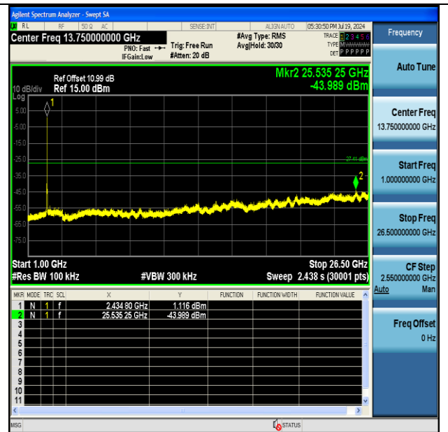
11N20SISO-Ant1-2437-1000~26500-PASS
